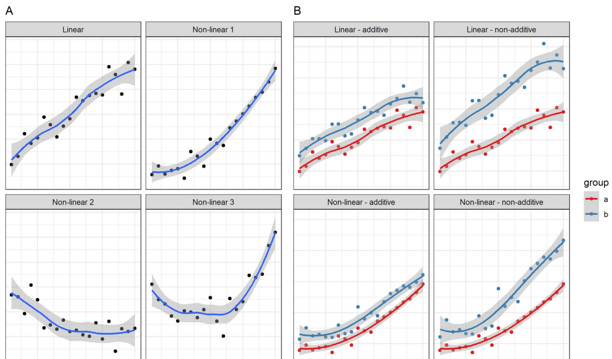
Fig. 1 Illustration of different types of relationships. a , Various ways of how two variables can be related linearly (upper left subpanel) or nonlinearly (the other subpanels). The data on the x-axis is an arbitrarily chosen range of numbers, and the relationship with the y-data was artificially simulated, including some noise (random error). b , the concept of nonadditivity. The upper two subpanels show for a linear relationship how the effect of group (color) can be additive (left) or nonadditive (right) over the x-variable. The bottom subpanels show the same for a nonlinear relationship
