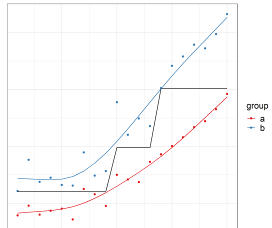
Fig. 2 Fitting a regression model ( lm function in R) and a regression tree ( rpart function in R) to the nonadditive, nonlinear relationship shown in Fig. 1b, bottom right subpanel. Again, the data shown on the x-axis was an arbitrarily chosen range of numbers, and the y-data were artificially simulated, including some noise (random error). The regression model (in colored lines) included a restricted cubic spline and an interaction term between group and x and follows the relationship nicely. The regression tree (black line) failed to include group in the final tree and only included x, thereby disregarding complexity in the data
