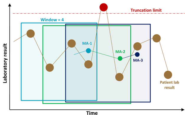
Figure 1: The principle of moving average quality control (MA QC). The average of a specific number of patient results is continuously calculated (in this example the four most recent patient results, as the window is set on 4). Each time a new patient result is generated, a new moving average value is calculated (depicted as MA-1, MA-2, and MA-3). Patient results above the truncation limit are excluded from the moving average calculation (depicted in red).
