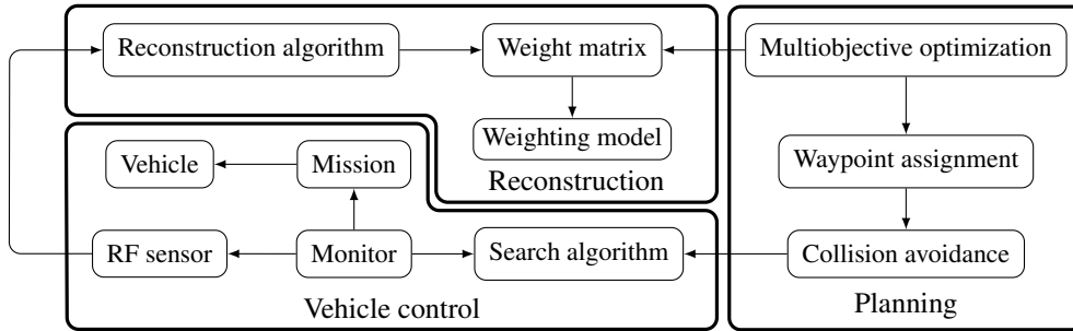
Figure 2: Diagram of components in the toolchain.
