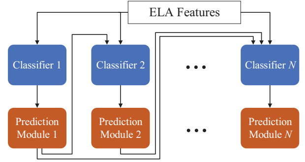
Fig. 1. Schematic representation of a Classifier Chain.
