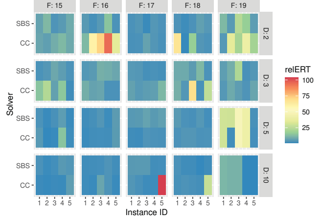
Fig. 4. Performance (in terms of the relative ERT) of the SBS and CC (with costs for ELA features), shown for the functions of BBOB function group 4.
