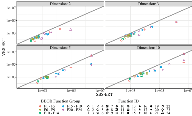
Fig. 2. Performance gap of the SBS and VBS.
