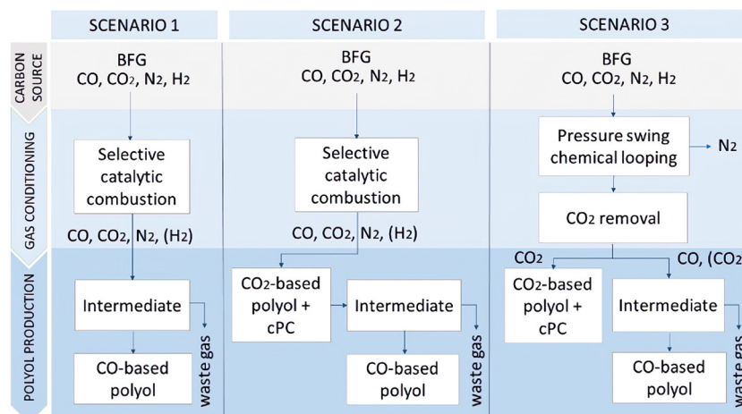
Fig. 2 Overview of scenarios of the CCU technology.
