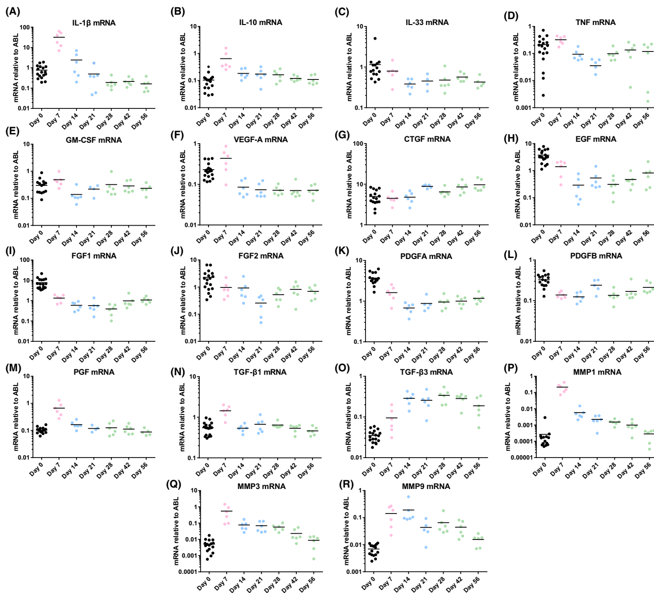
FIGURE 4 mRNA expressing quantified using qPCR. Data is expressed as individual data points with means, relative to housekeeping gene ABL ( n=18 for day 0, n=6 for all other timepoints). Colour coding corresponds to wound healing phases depicted in Figure 1A. Black=pre-challenged skin, pink=inflammation phase, blue=proliferation phase, green=remodeling phase. Data are expressed as means.
