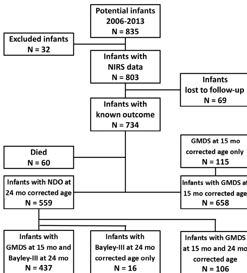
Figure 1. Flow chart of included patients. NDO , neurodevelopmental outcome.
