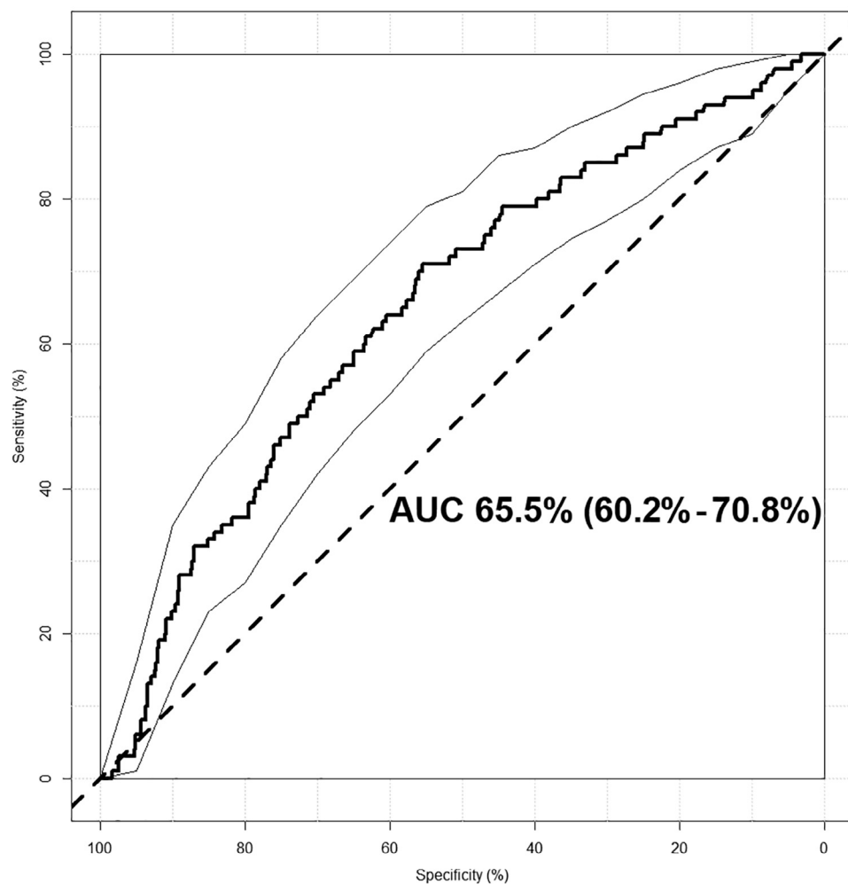
Figure 4. ROC curve with 95% CI for time spent <55% 0-72 hours after birth with composite cognitive outcome at 24 months of corrected age. AUC, area under the curve.
