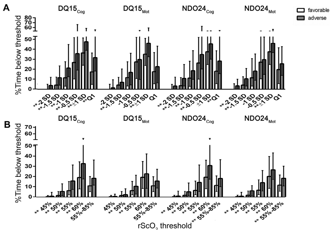
Figure 3. The percentage of A , time spent below and outside thresholds based on published reference values, and B , time spent below or outside fixed thresholds during 0-72 hours after birth for outcomes at 15 and 24 months of corrected age. Q1, time spent with rScO_2 in the lowest quartile based on the current data set. ** Indicates statistical significance based on Mann-Whitney U test or Student t test, where applicable.
