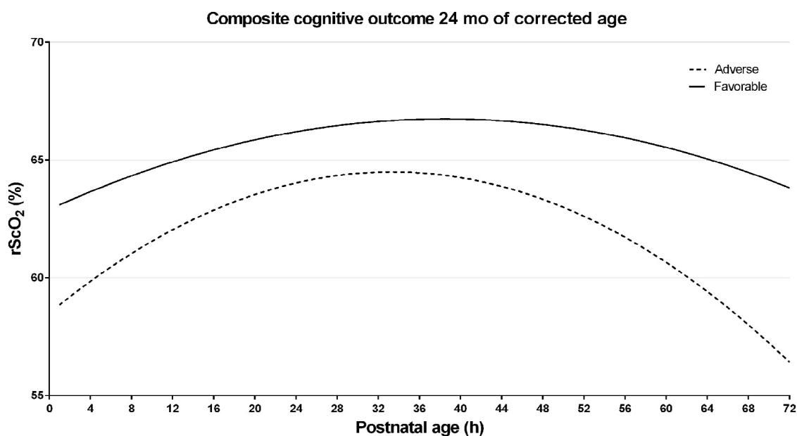
Figure 2. The model fit of the course of the rScO_2 over time plotted for infants with adverse and favorable outcome.
