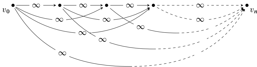
Figure 5. The graph M_n of C(\mathbb{CP}_q^n) .
