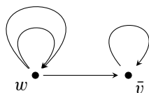
Figure 1. The graph \Lambda .
