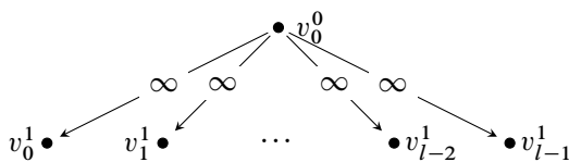
Figure 8. The graph W_l of C(\mathbb{W}P_q^1(1, l)) .
