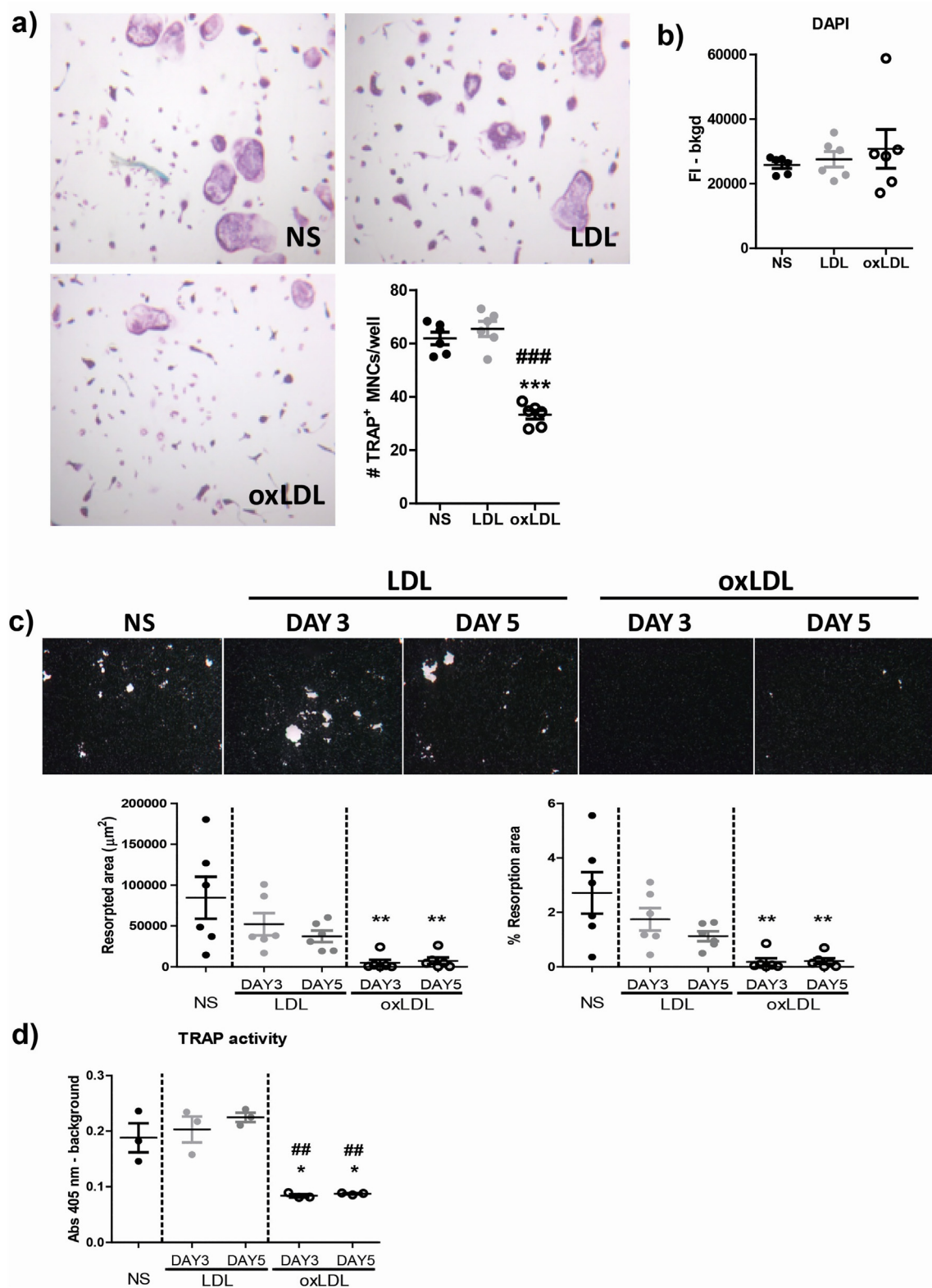
Fig. 5. oxLDL strongly restrains the formation of multinucleated osteoclasts and their resorptive activity at a later stage of differentiation. Wild-type (WT) multinucleated osteoclasts were stimulated with 10 µg/ml LDL or oxLDL for 24 h. a) Representative photomicrographs and quantification of TRAP positive (TRAP + ) cells show a strong inhibition of osteoclastogenesis upon oxLDL, but not LDL stimulation. Original magnification, 100× b) Note that oxLDL did not affect cell viability as determined by fluorescence intensity (FI) signals of DAPI stain (n = 6 mice). c) Representative photomicrographs and quantification of resorption on biomimetic hydroxyapatite-like-coated plates show a significant reduction of pit areas upon exposure of both pre-osteoclasts (day 3) and multinucleated osteoclasts (day 5) to oxLDL; of note, exposure to LDL reduced pit formation, though this reduction was not significant (n = 6 mice). Original magnification, 100× d) Finally, TRAP activity in the culture supernatants of WT mature osteoclasts was strongly down-regulated both upon exposure of pre-osteoclasts (day 3) and multinucleated osteoclasts (day 5) to oxLDL, but not LDL (n = 3 mice). Error bars represent the mean ± SEM. (* = P < 0.05 , ** = P < 0.01 , *** = P < 0.001 compared to NS controls; ## = P < 0.01 , ### = P < 0.001 compared to LDL stimulated samples).
