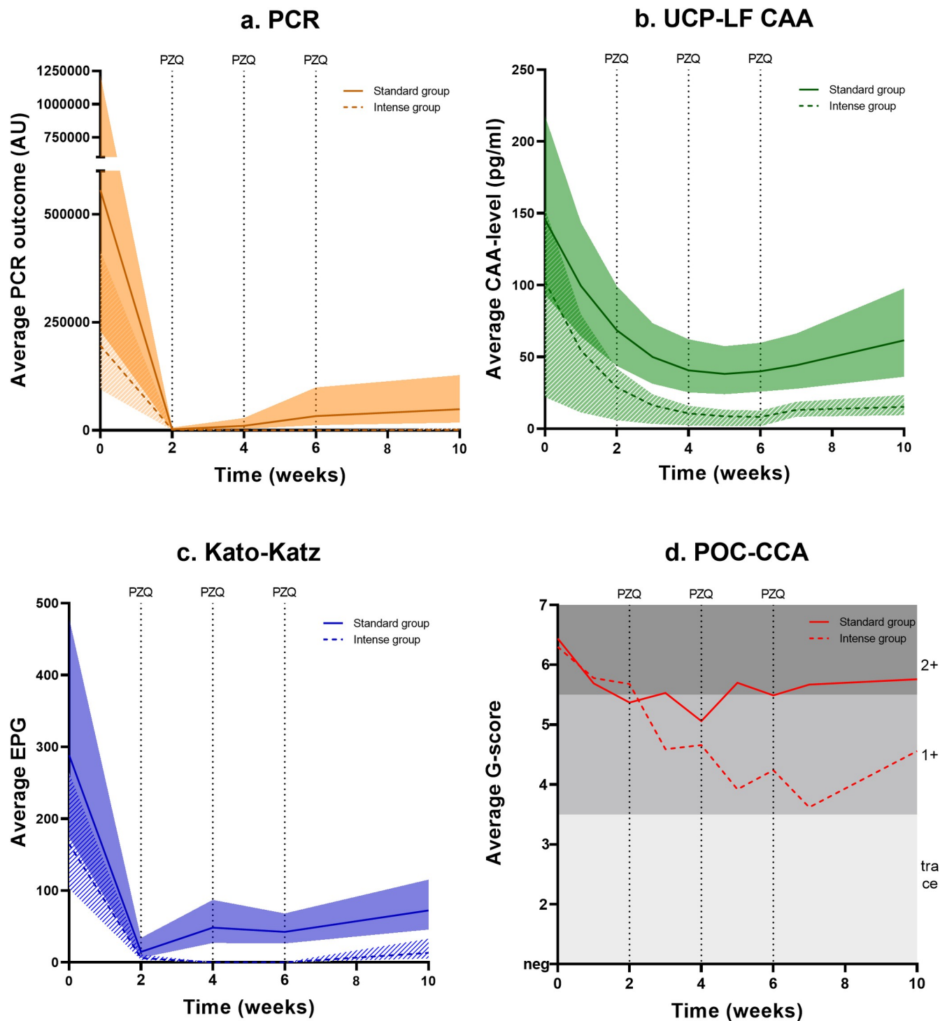
Fig 2. Average infection levels over time with corresponding 95% confidence intervals* estimated from the mixed effects logistic regression model. Data shown for (a) polymerase chain reaction (PCR), (b) up-converting particle circulating anodic antigen (UCP-LF CAA), (c) Kato-Katz (KK), and (d) point-of-care circulating cathodic antigen (POC-CCA), in the standard treatment group ( n = 56 , single dose of PZQ at week 0, solid line) and intense treatment group ( n = 69 , four doses of PZQ at weeks 0, 2, 4, and 6, dashed line). *for POC-CCA no confidence intervals available.
