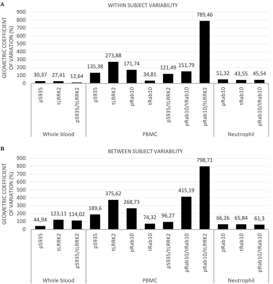
Figure 2 Variability of each biomarker in each biological source. A. Within-subject (intrasubject) variability between VISITS 1 and 2. B. Between-subject (intersubject) variability of pS935, tLRRK2, pS935/tLRRK2, pRab10, tRab10, pRab10/tRab10, and pRab10/tLRRK2 in whole blood, PBMCs and neutrophils expressed as geometric coefficient of variation (%). Data from all 3 subpopulations (LRRK2+PD, iPD, and HC) was pooled for this analysis. Within-subject and between-subject variability were low in whole blood and neutrophils, and substantially higher in PBMCs. Supplemental Figure S2A-F for a breakdown per subpopulation.
