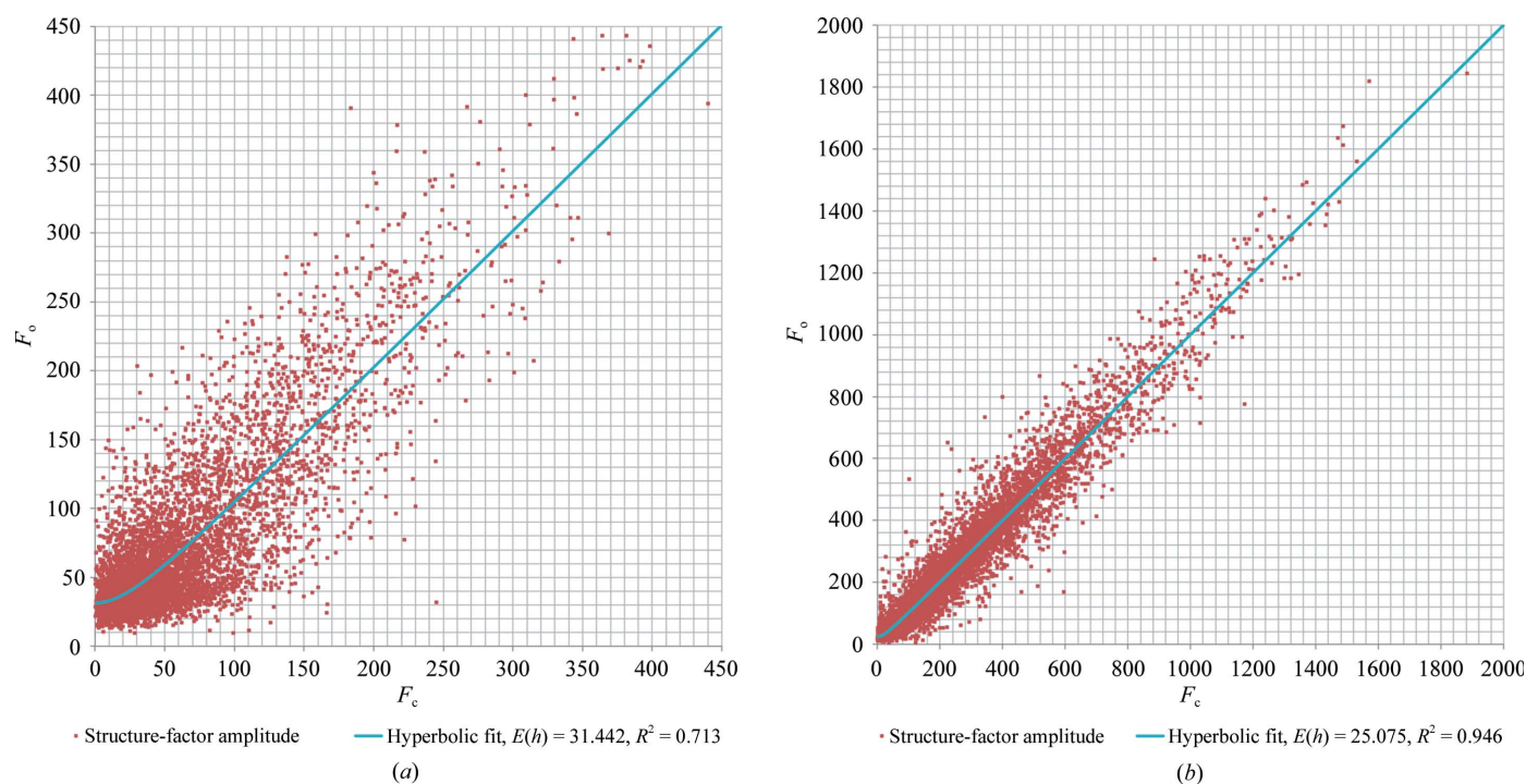
Figure 6 F_o versus F_c graphs for (a) electron diffraction of a single lysozyme nanocrystal and (b) an X-ray data set for cubic (bovine) insulin at 1.6 Å resolution. The data were least-squares fitted with a hyperbolic function described by \langle |F_o| \rangle = [F_c^2 + \langle |E(h)| \rangle^2]^{1/2} . F_o versus F_c graphs for only the low-resolution part of the single-crystal data and for the merged crystal data are shown in Supplementary Fig. S6.
