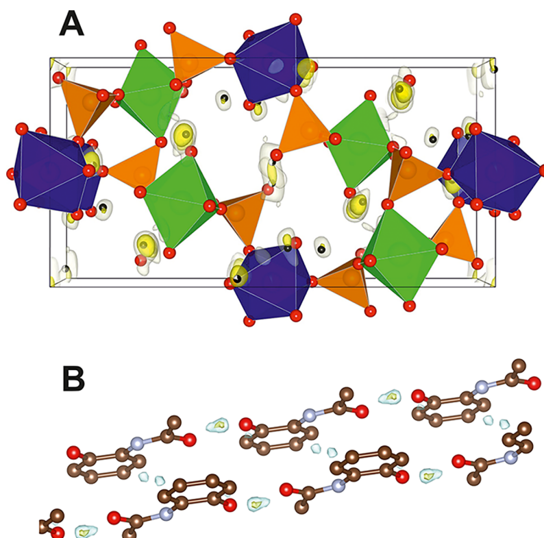
Figure 5. Hydrogen atoms localization by 3D ED. (A) Perspective view of the \text{Co}_{1.13}\text{Al}_2\text{P}_4\text{O}_{20}\text{H}_{11.74} structure 105 with a superimposed difference potential map showing maxima at the positions of the hydrogen atoms. Isosurface levels are at 2\sigma[\Delta V(r)] (light gray) and 3\sigma[\Delta V(r)] (yellow). \text{CoO}_6 , \text{AlO}_6 , and \text{PO}_4 polyhedra are represented in blue, green, and orange, respectively, while oxygen atoms are in red. This difference potential map enlightening the hydrogen positions is obtained thanks to the use of dynamical refinement. The hydrogen positions (in black) are stable once incorporated to the dynamical refinement. (B) Two adjacent orthocetamol chains 34 with the superimposed difference Fourier map. The maximum residual potential (in blue and yellow) corresponds to the hydrogen atom responsible for the intermolecular bonding. Carbon atoms are drawn in brown, oxygen atoms in red, and nitrogen atoms in gray.
