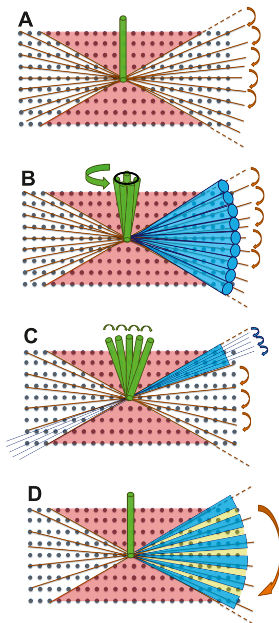
Figure 2. Sketches of the four main 3D ED data collection protocols. (A) Simple stepwise acquisition performed with fixed mechanical tilt steps (brown arrows) and steady beam (in green). The tilt step is normally 0.5\text{--}2^\circ . (B) Stepwise acquisition performed with fixed mechanical tilt steps (brown arrows) while the beam is precessing around a conical surface pointed on the sample (green arrow). The Ewald sphere is also precessing (blue cones), and this movement allows a better integration of the Bragg reflection intensities. (C) Stepwise RED acquisition. Large mechanical tilt steps (brown arrows) are followed by small beam tilt steps (green arrows) obtained by the deflection coils of the TEM. The beam tilt step may be smaller than 0.1^\circ . (D) Continuous rotation acquisition. The sample is mechanically tilted within the whole goniometer range (brown arrow) while the detector is acquiring a sequence of patterns. The acquisition tilt step is determined by the sum of exposure time (blue) and readout time (yellow). The latter is also responsible for the nonsampled wedges between two consecutive patterns. The beam is stationary during the whole data acquisition, and the main limit is given by the goniometer stability, because the sample tends to shift laterally during the tilt and therefore may go out from the illuminated area. The not sampled missing wedge is exaggerated in the figures and is colored in red. It is the same for all acquisition protocols, as it depends only on the mechanical limit of the TEM goniometer.
