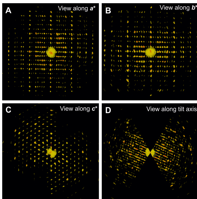
Figure 3. Exemplary diffraction volume of the trigonal mineral franzinite reconstructed from 3D ED data ( a = 12.9 \text{ \AA} , c = 26.6 \text{ \AA} ). (A) View along a^* . (B) View along b^* . (C) View along c^* . (D) View along the tilt axis of the acquisition. Note that these are projections of a 3D volume and not conventional 2D oriented ED patterns. Cell edges are sketched in yellow. a^* vector is in red, b^* vector in green, and c^* vector in blue. Data resolution is about 0.8 \text{ \AA} . The figure is made by ADT3D software. 18
