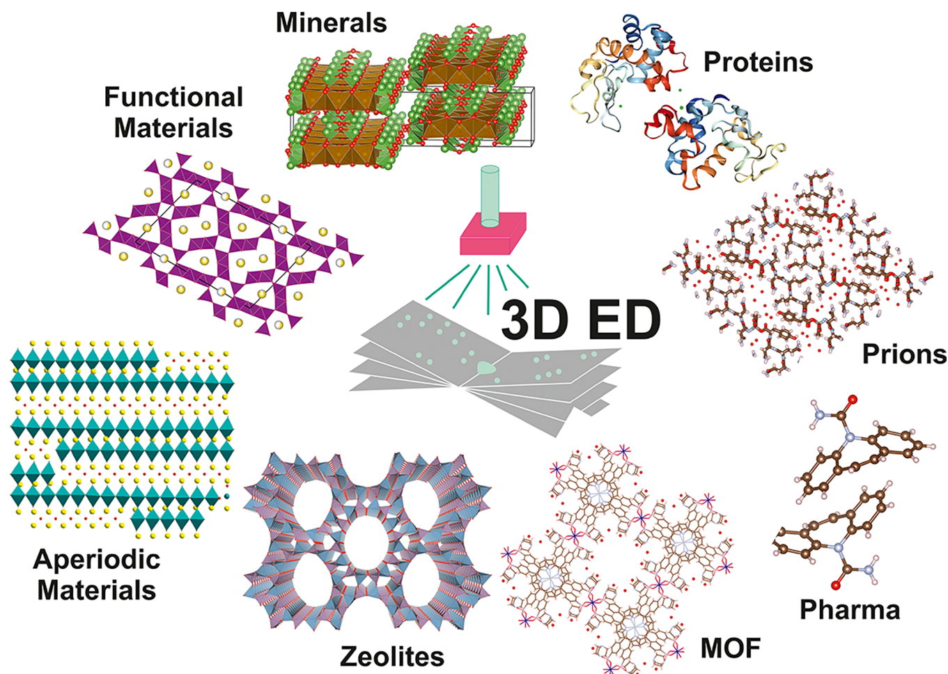
Figure 4. Sketch showing some representative structures solved by 3D ED method for different classes of materials. Starting from the upper left and going anticlockwise: the mineral karibibite, 133 a tunnel (Na,Mn)-oxide for electrolytic applications, 124 the aperiodic structure of \text{SrBi}_7\text{NbO}_{24} , 122 the extra-large-pore silicoaluminophosphate ITQ-51, 25 the cobalt tetraphosphonate MOF Co-CAU-36, 66 the pharma compound carbamazepine-III, 29 the amyloid core of the Sup35 prion protein, 47 and a new monoclinic polymorph of lysozyme. 45
