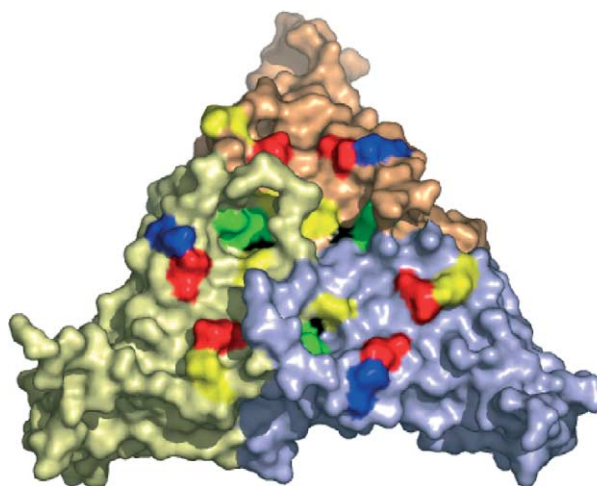
Figure 5. Surface representation of subunits A (orange), B (yellow) and C (blue) viewed along the quasi 3-fold axis from the interior of the capsid. The histidine 68 and histidine 180 (green) are located close to the interface between subunits A, B and C. The cavities containing histidine 68 and histidine 180 (green), accompanied by Arg67, Arg140 (yellow) and Asp143 (black) are surrounded by a Arg-Glu and a Lys-Glu couple (R12/E135 and K32/E72) (yellow/red and blue/red, respectively). The side-chain of these residues point towards the interior of the capsid.
