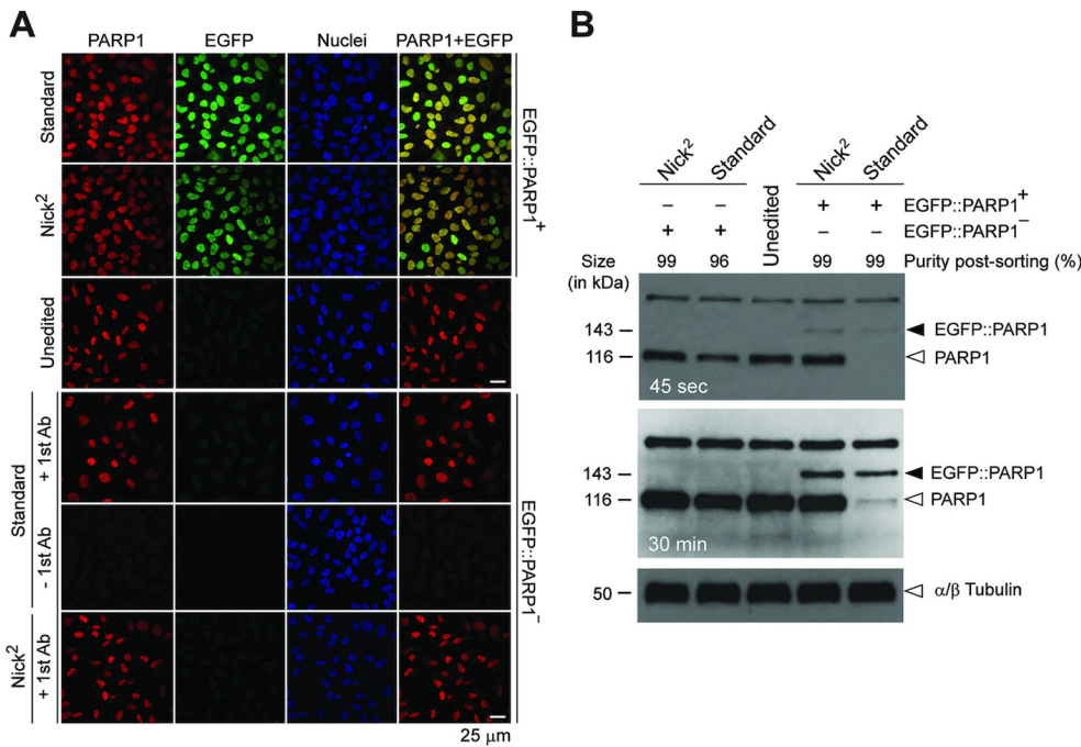
Figure 5. Examination of PARP1 protein status after gene editing triggered by DSBs versus SSBs. (A) Confocal microscopy analysis of HeLa cells expressing untagged and EGFP-tagged PARP1. Confocal microscopy of EGFP::PARP1 + and EGFP::PARP1 - cells confirming co-localization of PARP1 and EGFP in the nuclei of the former cell populations engineered by in trans paired nicking or standard gene editing. Nuclei were counterstained with DAPI. Unedited HeLa cells served as negative controls. Specimens of EGFP::PARP1 - cells not incubated with the primary PARP1-specific antibody (-1st Ab) provided for an additional staining control. (B) Western blot analysis of HeLa cells expressing untagged and EGFP-tagged PARP1. Western blotting of EGFP::PARP1 + and EGFP::PARP1 - cells exposing a striking reduction in the amounts of endogenous PARP1 antigen exclusively in EGFP::PARP1 + cells generated through standard DSB-dependent gene editing (open arrowhead). Properly sized EGFP::PARP1 fusion products were detected in both EGFP::PARP1 + cell populations (solid arrowhead). Unedited HeLa cells served as negative controls. α/β Tubulin antigens served as internal protein loading controls.
