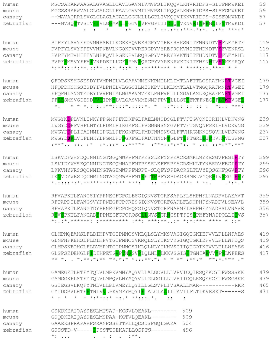
Fig. 5. Multiple species sequence alignments of SCARB1 (A) Alignments of SCARB1 sequences were generated using the Clustal Omega alignment program (EMBL-EBI). Three known human SCARB1 mutation locations (rs397514572 [p.Ser112Phe], rs187831231 [p.Thr175Ala], rs387906791 [p.Pro297Ser]) as well as the Arg-174 and Asp-185 are highlighted in magenta. The amino acids that differ in only in zebrafish are highlighted in green. An asterisk (*) indicates positions which have a fully conserved residue. A colon (:) indicates conservation between sequences that have strong similar properties. A period (.) indicates conservation between sequences that have weak similar properties. (For interpretation of the references to colour in this figure legend, the reader is referred to the web version of this article.)
