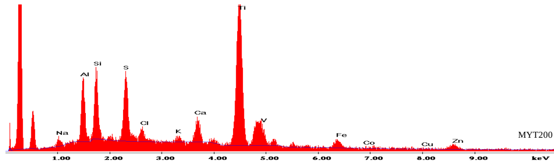
Figure 157 Purple pigments. Graphs from Mytilene samples.
