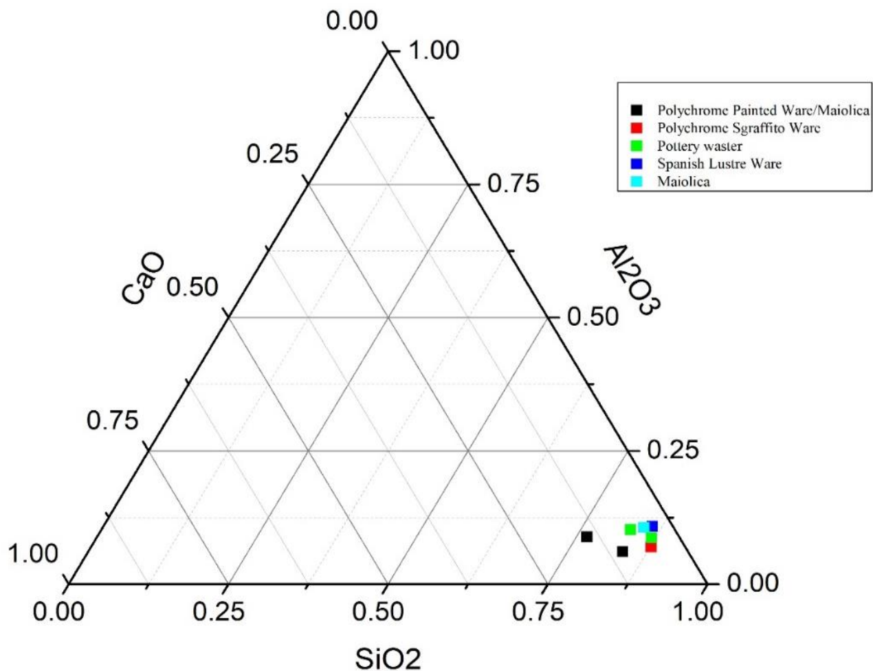
Figure 168 Correlation of the \text{SiO}_2 , \text{Al}_2\text{O}_3 , \text{CaO} for the glazes from the Athenian Agora in Attica through Scanning Electron Microscopy (SEM). The samples have been separated based on their pottery types.
