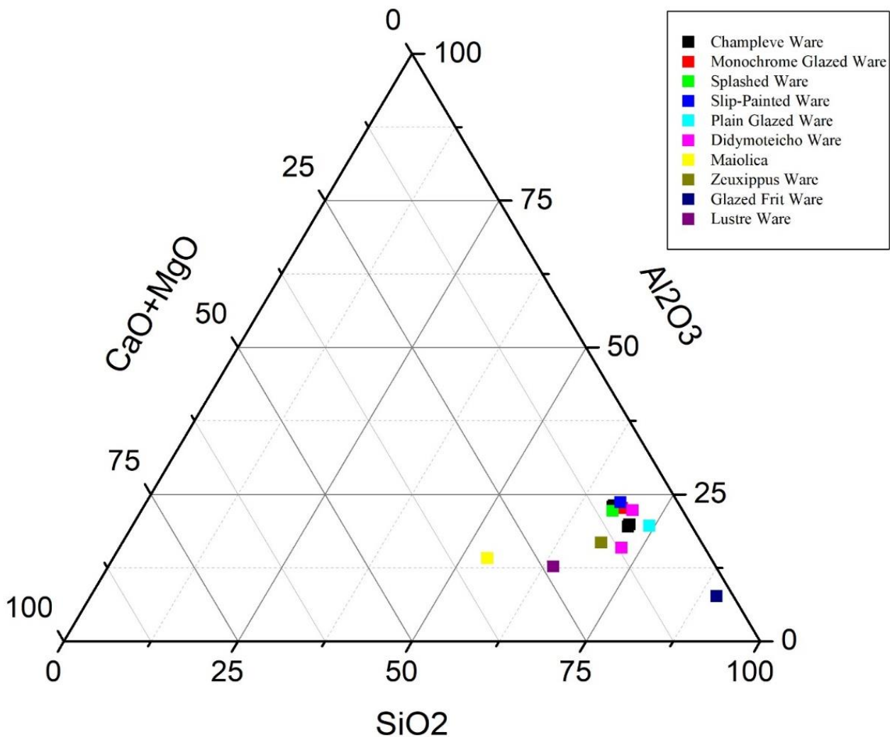
Figure 170 Correlation of the \text{SiO}_2 , \text{Al}_2\text{O}_3 , \text{CaO}+\text{MgO} for the fabrics from Chalcis in Euboea through Scanning Electron Microscopy (SEM). The samples have been separated based on their pottery types.
