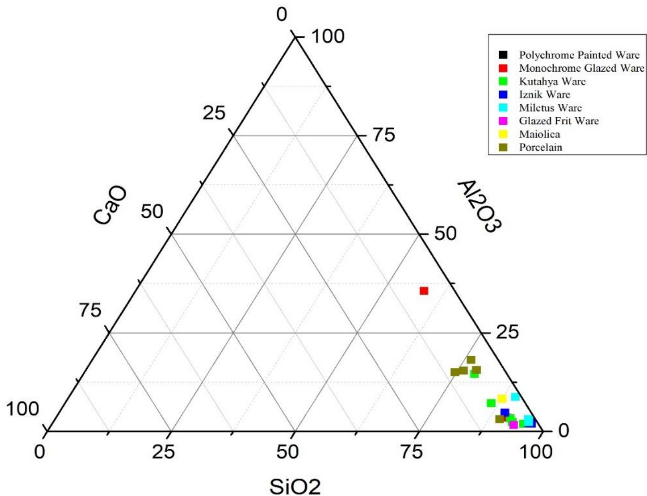
Figure 169 Correlation of the \text{SiO}_2 , \text{Al}_2\text{O}_3 , \text{CaO} for the glazes from the Castle of Mytilene in Lesvos through Scanning Electron Microscopy (SEM). The samples have been separated based on their pottery types.
