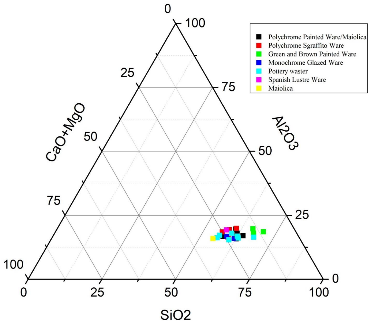
Figure 171 Correlation of the \text{SiO}_2 , \text{Al}_2\text{O}_3 , \text{CaO}+\text{MgO} for the fabrics from the Athenian Agora in Attica through Scanning Electron Microscopy (SEM). The samples have been separated based on their pottery types.
