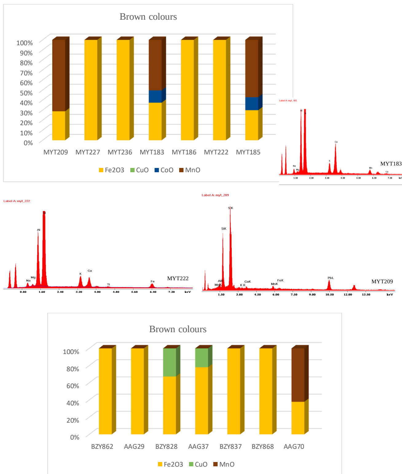
Figure 156 Brown pigments. Graphs from the pottery samples from the Castle of Mytilene in Lesbos samples (top, middle) and of the Athenian Agora in Attica (bottom).
