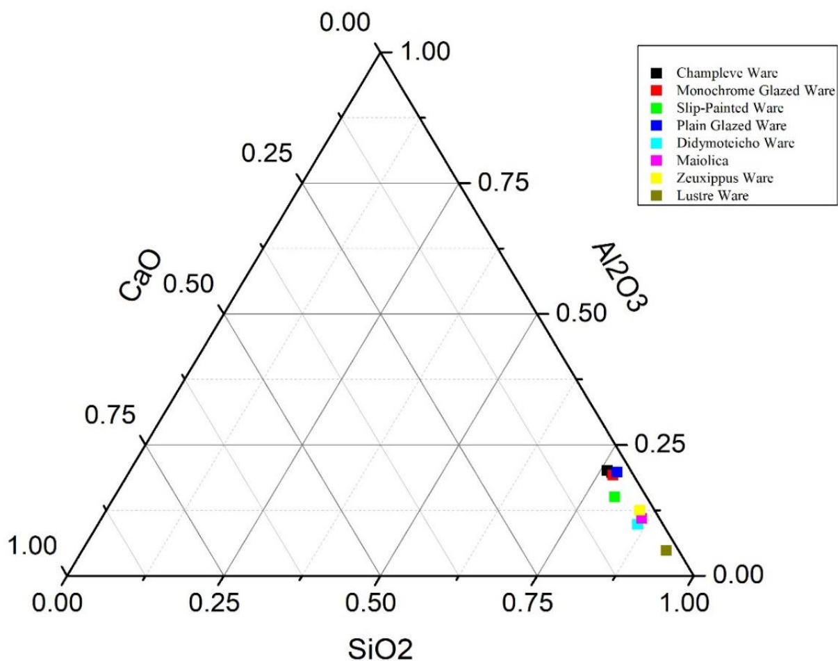
Figure 167 Correlation of the \text{SiO}_2 , \text{Al}_2\text{O}_3 , \text{CaO} for the glazes from Chalcis in Euboea through Scanning Electron Microscopy (SEM). The samples have been separated based on their pottery types.
