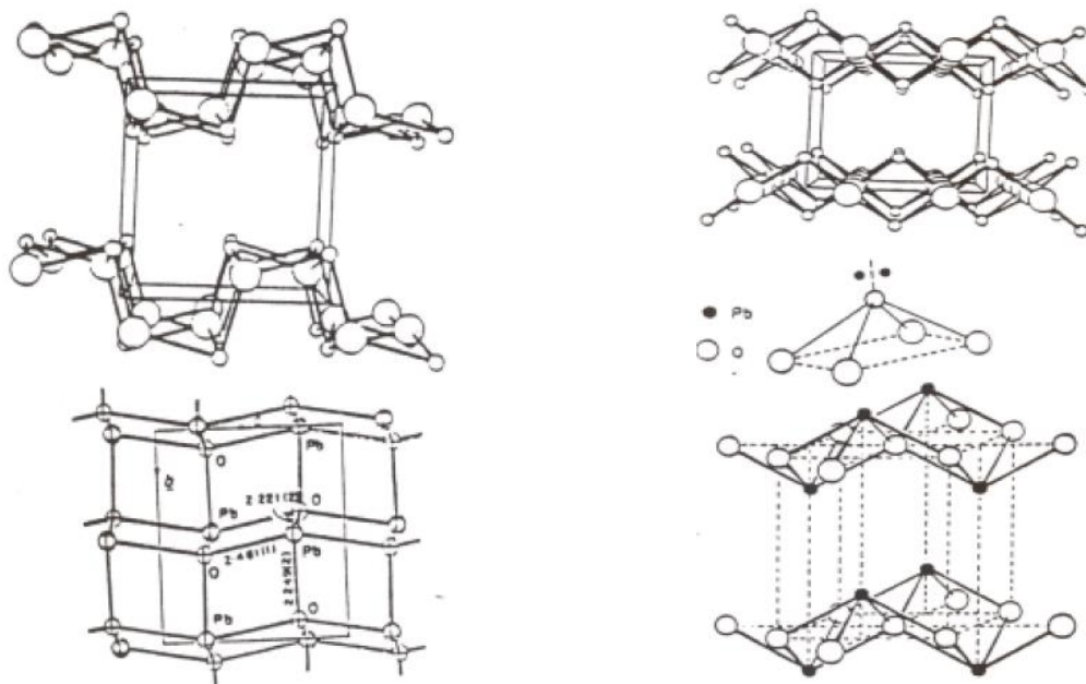
Figure 86 \alpha PbO, tetragonal known as litharge or red lead (Wells 1984; Fitch 2003, p. 184).
