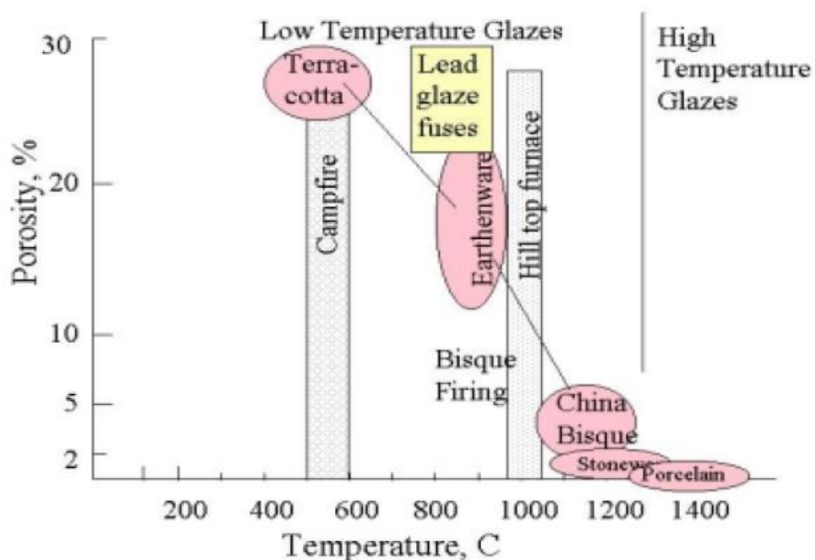
Figure 82 Porosity decreases with temperature. Very high temperatures are needed to remove the water from clay to achieve porcelain (Fitch 2003, p. 165).
