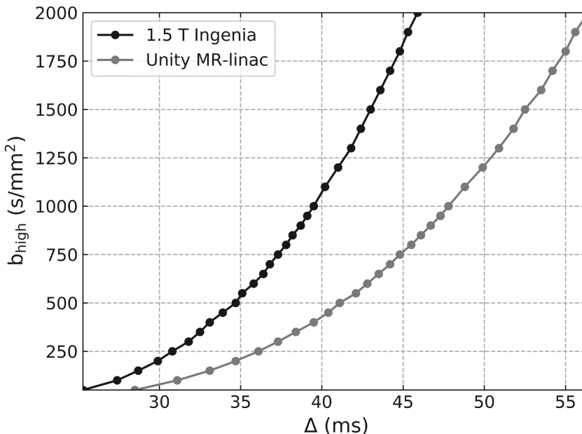
Figure 3.1. Comparison between the Unity system and a 1.5 T Philips Ingenia of the time between the start of the two diffusion gradients ( \Delta ). For example, a b-value of 1200 \text{s}/\text{mm}^2 at the diagnostic system has a \Delta of 41 ms. For the Unity system, the b-value with the same \Delta is less than half: 500 \text{s}/\text{mm}^2 .
