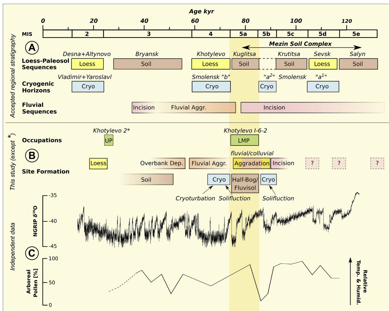
Fig. 9. (A) Accepted chronostratigraphy of the region compiled from Velichko (1990), Velichko et al. (2006, 2011, 2017) and Panin et al. (2017, 2018) compared with (B) findings of this study. Chronology for the occupation at Khotylevo 2 taken from Gavrilov et al. (2015)*. (C) NGRIP-data from North Greenland Ice Core Project members (2004), and Arboreal Pollen taken from Yelovicheva and Sanko (1999).
