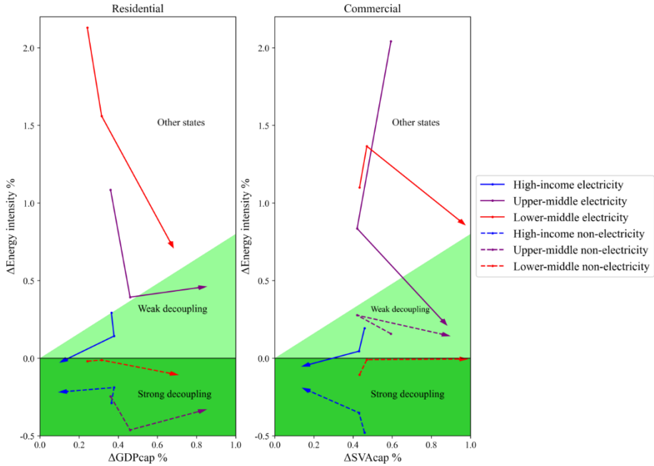
Figure 4.4 The state map of decoupling between energy intensity and economic development. Left: the change of the decoupling index (DI) of residential energy intensity ( \Delta E_{r/Fr} ) from GDP growth ( \Delta GDP_{cap} ); Right: the change of DI between commercial energy intensity ( \Delta E_{c/Fc} ) and Service Value Added growth ( \Delta SVA_{cap} ). Each line shows three data points representing the time periods of 1971-1985, 1985-2000, 2000-2014, respectively. The changing directions in all groups (blue for high-income, purple for upper-middle-income, red for lower-middle-income) are shown by the arrows. The solid lines represent the electricity intensity and the dashed lines represent the non-electricity energy.
