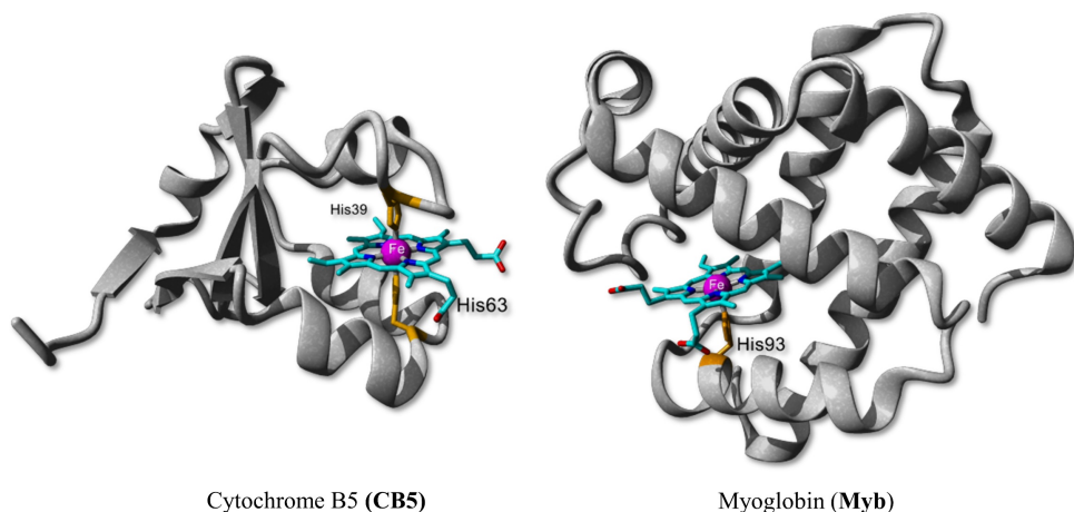
Figure 2.3. Haem proteins used to produce ArMs as WOC: Cytochrome B5 ( CB5 , left, PDB:1CYO) and Myoglobin ( Myb , right, 5D5R). The proteins are shown with the natural haem cofactor in the binding pocket, and the metal-binding histidines residues coloured in orange.
