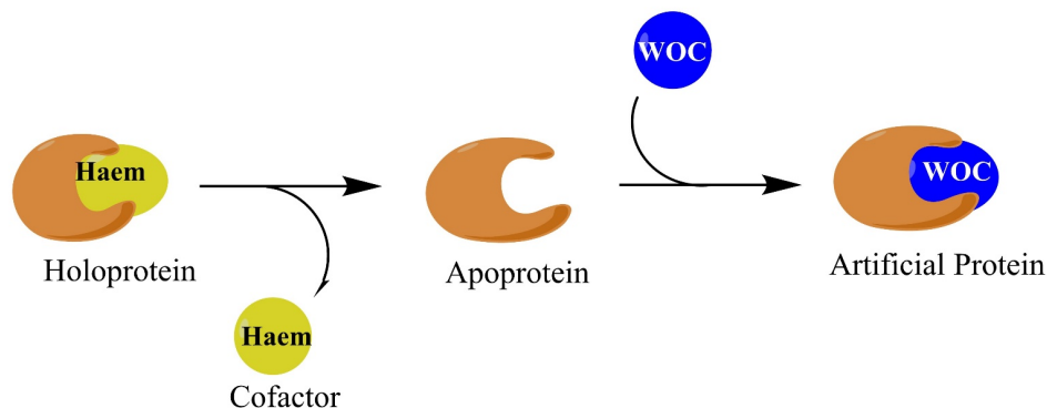
Figure 2.1. Representation of the strategy used on this chapter to prepare a water-oxidizing artificial protein.
