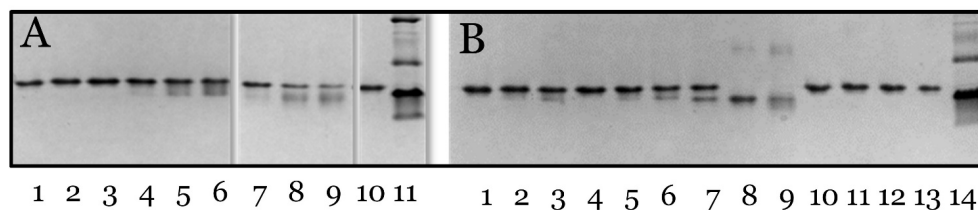
Figure 2.5. Semi-native SDS-gel electrophoresis analysis of the reaction between apoCB5 and Ru1–Ru3 or Co1–Co4 complexes at increasing metal complex concentrations. (A) Ruthenium complexes: Lane 1 to 3, Ru1 ; Lane 4 to 6, Ru2 ; Lane 7 to 9, Ru3 ; Lane 10, apoCB5 ; Lane 11, protein reference ladder. (B) Cobalt complexes: Lane 1 to 3, Co1 ; Lane 4 to 6, Co2 ; Lane 7 to 9, Co3 ; Lane 10 to 12, Co4 ; Lane 13, apoCB5 ; Lane 14, protein reference ladder. Conditions: [Catalyst] = 10, 50 or 100 \mu\text{M} (from left to right for each complex), 200 \mu\text{L} samples were prepared in a 96-well plate, 20 mM phosphate buffer, pH 7.2, temperature 4 ^{\circ}\text{C} , in the dark, 3 days, [ apoCB5 ]=10 \mu\text{M} .
