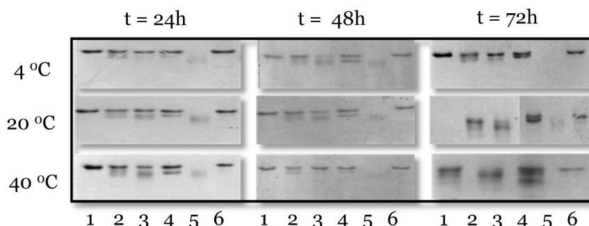
Figure 2.7. Temperature screening of the reaction between apoCB5 and Ru- and Co-complexes using SDS semi-native gel. Lane 1, Ru1 ; Lane 2, Ru2 ; Lane 3, Ru3 ; Lane 4, Co2 ; Lane 5, Co3 ; Lane 6, Co4 . Conditions: 200 \mu L samples in a 96-well plate, 20 mM phosphate buffer, pH 7.2, in the dark, [ apoCB5 ] = 20 \mu M, [catalyst] = 200 \mu M.
