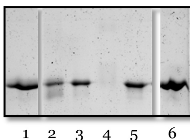
Figure 2.9. Semi–native SDS–gel of apoMyb and WOCs. Lanes: 1, Ru1 ; Lane 2, Ru2 ; Lane 3, Co1 ; Lane 4, Co3 ; Lane 5, Co4 ; Lane 6, apoMyb . Conditions: incubation 24 h at 4 °C, 20 mM phosphate buffer, pH 7, [ apoMyb ]=10 µM, [Catalyst]=100 µM.
