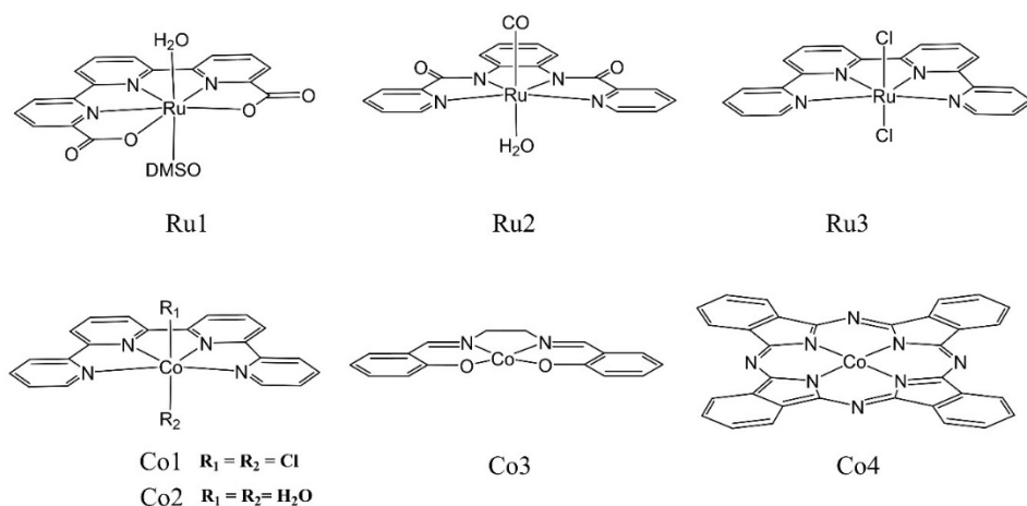
Figure 2.2. Ruthenium and cobalt complexes screened for the generation of a water-oxidizing artificial metalloenzyme.
