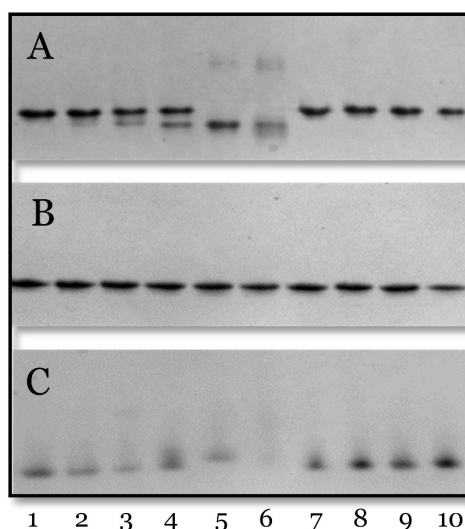
Figure 2.4. ArM formation between apoCB5 and cobalt complexes Co2 , Co3 , or Co4 , screened using semi-native (A), denaturing (B), or native (C) gel electrophoresis. Lane 1 to 3, Co2 ; Lane 4 to 6, Co3 ; lane 7 to 9, Co4 ; Lane 10 is apoCB5 . Concentration of the cobalt complex is 10, 50 or 100 \mu\text{M} from left to right for each complex set. Conditions: 20 mM phosphate buffer, pH 7.2, temperature 4 ^{\circ}\text{C} , in the dark, reaction time = 3 days, [ apoCB5 ]=10 \mu\text{M} .
