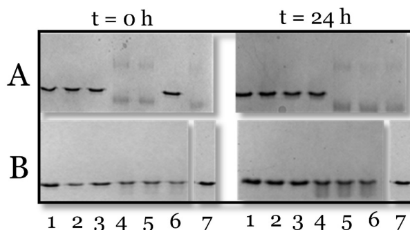
Figure 2.8. Influence of the reaction time on the reaction between apoCB5 and Ru1–Ru2 or Co2–Co3 according to SDS semi-native gel. (A) at t = 0 h, Lane 1 to 3, Co2 (triplicate); Lane 4, 5 and 7, Co3 (triplicate); Lane 6, apoCB5 . At t = 24 h, Lane 1, apoCB5 ; Lane 2 to 4, Co2 (triplicate); Lane 5 to 7, Co3 (triplicate). (B) for both gels; Lane 1 to 3, Ru1 (triplicate); Lane 4 to 6, Ru2 (triplicate); Lane 7, apoCB5 . Conditions: 200 \mu L samples were prepared in a 96-well plate by, 20 mM phosphate buffer, pH 7.2, temperature 4 ^{\circ} C, in the dark, [ apoCB5 ]=10 \mu M, [catalyst]=200 \mu M.
