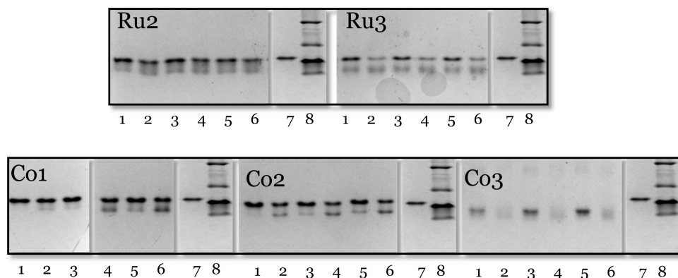
Figure 2.6. Effect of pH on the binding of ruthenium (top) and cobalt (bottom) complexes to apoCB5 according to semi-native SDS-gel. For each gel: complex concentration 100 \mu\text{M} (Lane 1,3 and 5) and 200 \mu\text{M} (Lane 2,4 and 6); Lane 1 and 2, pH 6; Lane 3 and 4, pH 7; Lane 5 and 6, pH 8; Lane 7, apoCB5 ; Lane 8, ladder. Conditions: 200 \mu\text{L} samples were prepared in a 96-well plate, 20 mM phosphate buffer, temperature 4 ^{\circ}\text{C} , in the dark, 3 days, [ apoCB5 ]=10 \mu\text{M} .
