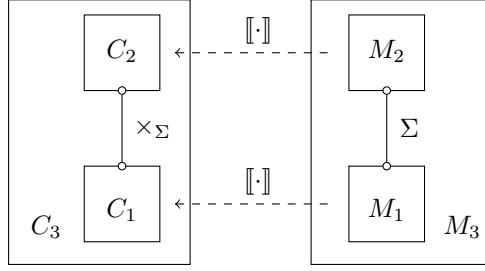
Figure 1.1: Two machines M_1 and M_2 , whose respective behavior is captured by C_1 and C_2 , interact through a protocol \Sigma . The product of the two components under the operation \times_\Sigma reflects the behavior of the machines interacting with the protocol \Sigma .
