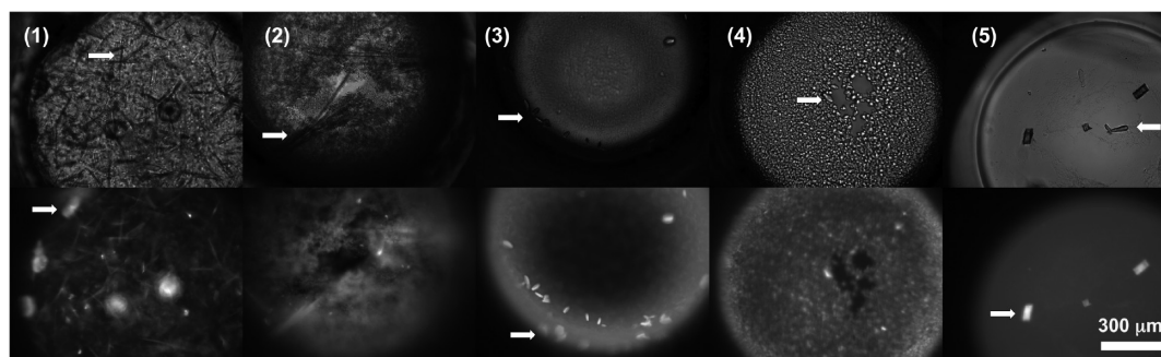
Figure 4. Bright field (above) and UV (below) images of protein crystals suspected of being false positives. In the bright field images the arrows point to the suspected crystals in the UV these crystals fluoresce. In the UV images the arrows point to fluorescent hair slices. 1. The small needles are glucose isomerase crystals. 2. Crystals of alpha lactoglobulin at right and bottom left, under a cloud of precipitation. 3. Small crystalline discs of alcohol dehydrogenase around bottom edge of plate where hair (bigger discs) are also present. 4. Small crystals of insulin, the biggest crystals fluoresce the most in UV light. 5. Salt crystals; these crystals do not fluoresce.
