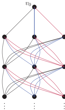
FIGURE 5 The Bratteli diagram of F_{(012)} with incoming edges ordered left to right.
