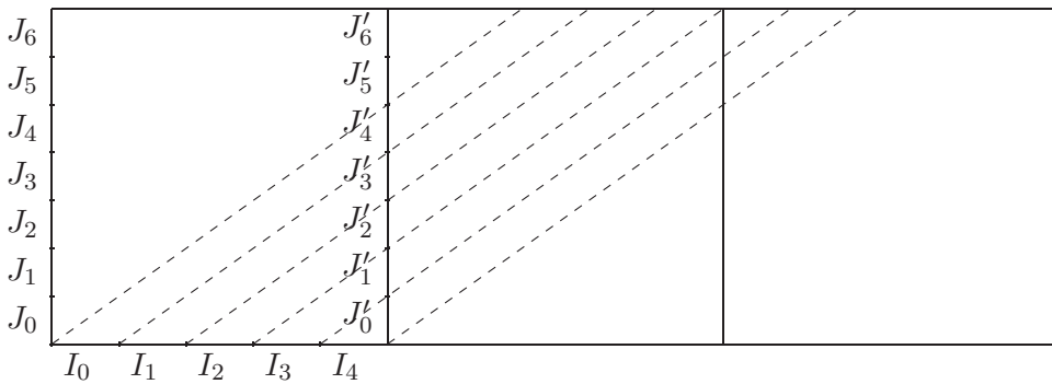
FIGURE 4 The flow for the rotation by \frac{2}{5} , so q = 5 , p = 7 , and r = 2 ; if the vertical edges are identified by a single translation, like in the torus, then the corresponding permutation of \{I_k\}_{k=0}^4 is \pi = (02413) . Identifications of the vertical sides using a nontrivial permutation \pi' of \{J'_k\}_{k=0}^6 may result in a different \pi . When gluing the vertical edges using a nontrivial \pi' , we have to remove the endpoints of the intervals in \{J'_k\}_{k=0}^6 from S , possibly creating planar ends in the resulting surface.
