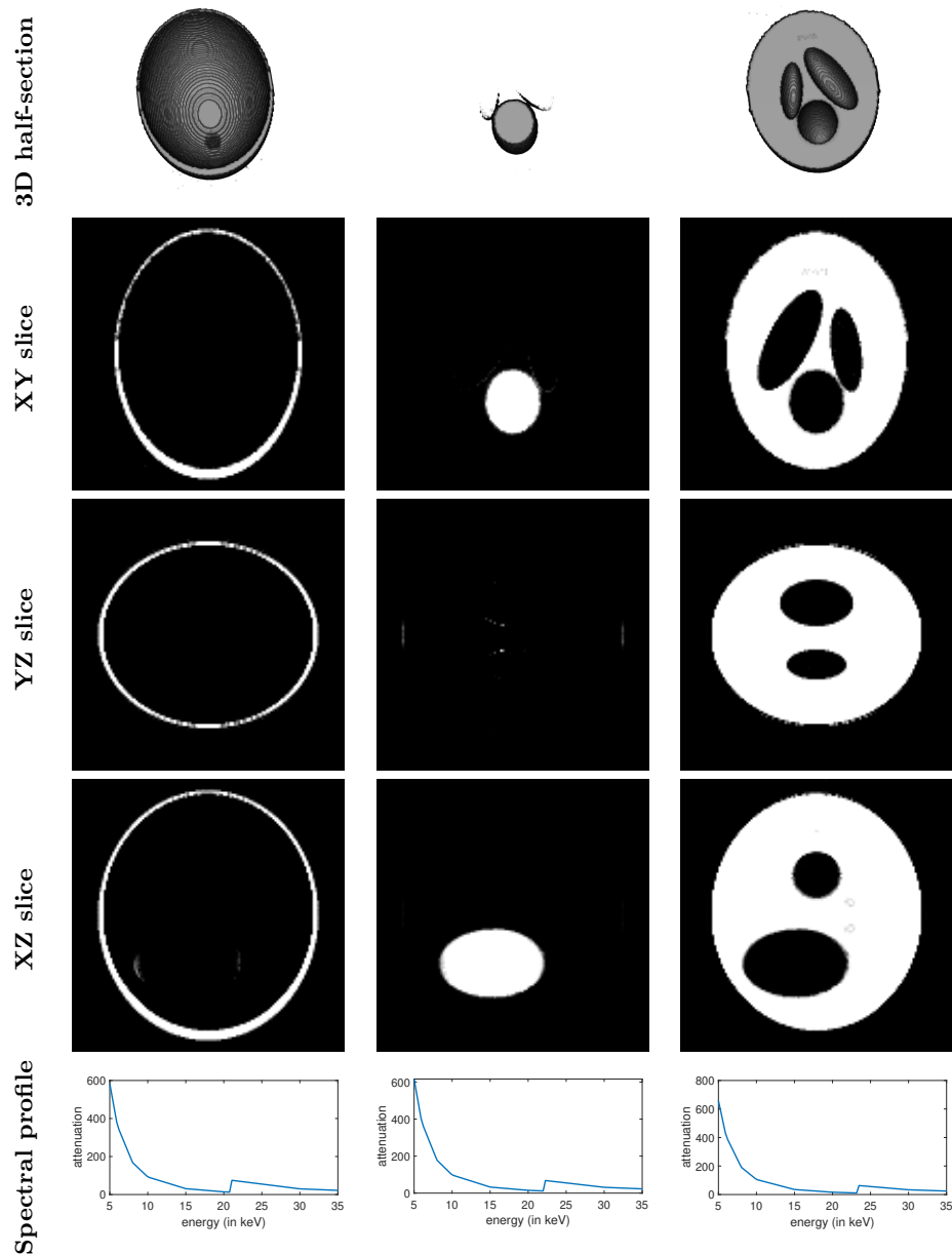
Figure A9: The reconstructed material composition of the 3D Shepp-Logan phantom from ADJUST algorithm. The materials contained in this phantom are vanadium (left column), chromium (middle column), and manganese (right column).
