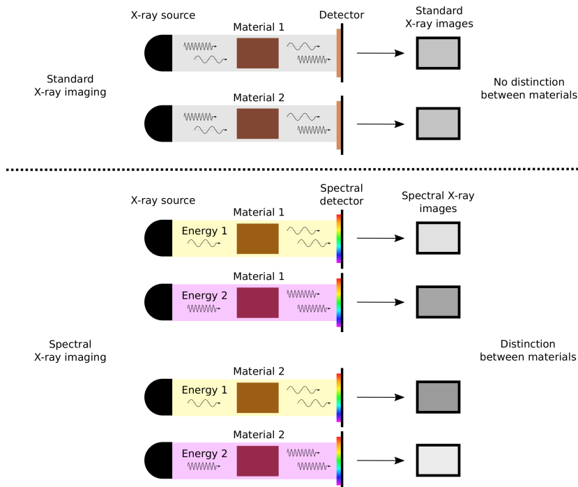
Figuur S1: Schematic representation of the advantage of spectral X-ray imaging over standard X-ray imaging. With standard X-ray imaging, two different materials can result in the same intensity on the X-ray image. With spectral X-ray imaging, the energies in the X-ray beam can be separated from each other (by adjusting the source, or by measuring both energies in a spectral detector, or both). This gives multiple X-ray images per material. Based on the differences in these spectral X-ray images between materials, we can distinguish them.
