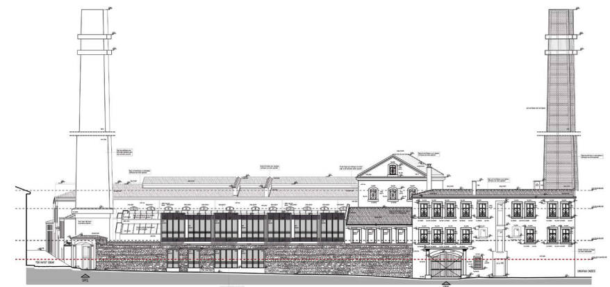
Figure 15: Restoration project, façade
