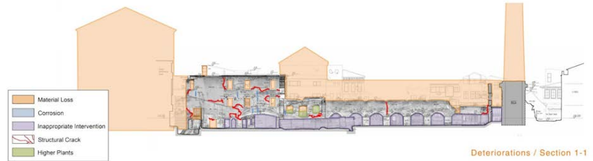
Figure 2: Unkapanı Flour Mill deteriorations in elevation (Modified from Alper, 2021)
