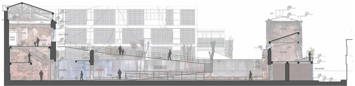
Figure 9: Longitudinal section showing the relation between the historic buildings, the ramp, and the courtyard
