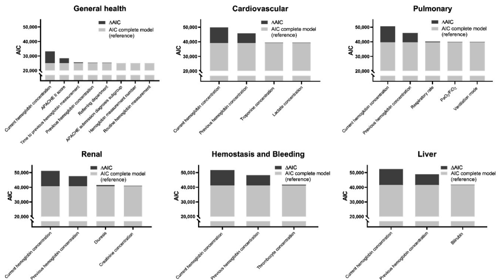
Fig. 2 Change in Akaike information criterion after excluding the single predictor from the multivariable model containing all variables of the organ system a . Only variables with \Delta AIC > 100 are presented.
