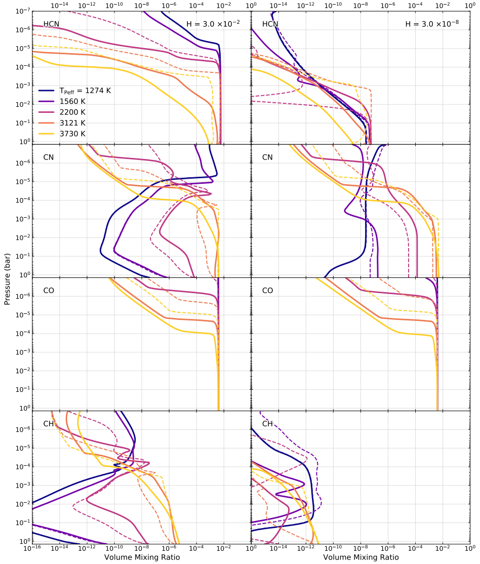
Figure 3.3: Volume mixing ratio of HCN, CN, CO and CH in nitrogen dominated hot super-Earth atmospheres. All cases shown for a C/O ratio of 2.5. Columns represent different hydrogen mass fractions, rows - different chemical compounds. The colour indicates the effective temperature of the planet. Solid lines represent atmospheres with temperature profiles shown in Figure 3.1, which in some cases have strong inversions. Dashed lines have CN and CH opacities omitted, hence lacking temperature inversions.
