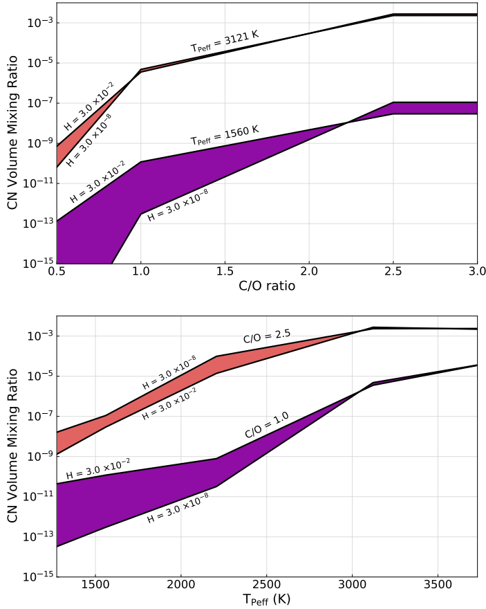
Figure 3.4: CN volume mixing ratio as a function of C/O ratio (upper panel) and T_{\text{Peff}} (lower panel). In the upper panel, different colours indicate different T_{\text{Peff}} . In the lower panel, different colours indicate different C/O ratios. For both panels, the spread indicates the effect of initial hydrogen abundance. The mixing ratios are averaged values of the 1.4 - 10^{-4} bar pressure region, which mostly coincides with the usual photospheric emission region. The temperature profiles used in these atmospheres are shown in Figure 3.1.
