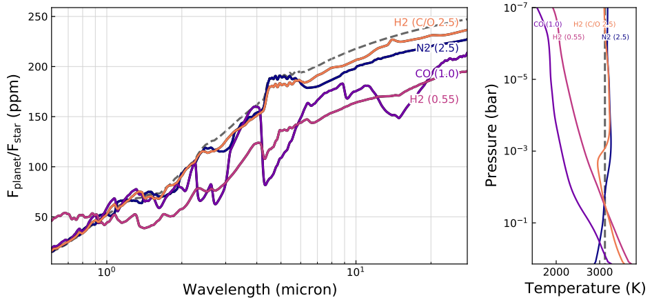
Figure 3.9: Comparison of synthetic emission spectra of atmospheres having different bulk compositions at T_{\text{Peff}} = 3121 K. The indicated numbers in brackets represent atmospheric C/O ratio. Exact compositions are listed in the lower subsection of 3.1. Corresponding temperature profiles are displayed in the panel on the right.
