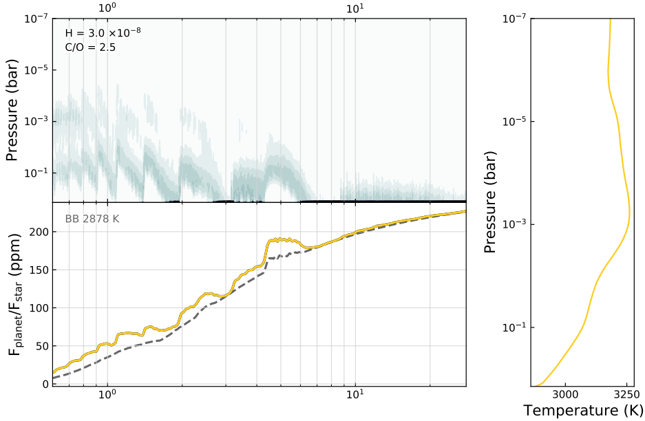
Figure 3.6: Contribution function of thermal emission of an atmosphere with an inverted thermal structure. The grey regions in the upper panel indicate the photosphere - optically thick regions being probed in emission. In the lower panel, indicated with yellow is a low resolution emission spectrum, with a coinciding surface temperature blackbody emission. The right panel indicates the corresponding temperature profile of the atmosphere.
