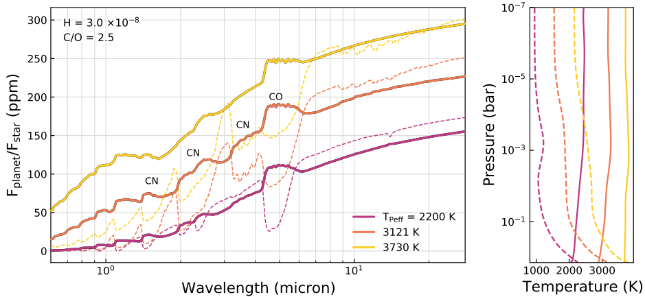
Figure 3.8: Emission spectra comparison between cases with temperature inversions and without. Same as in Fig. 3.7, but with depleted hydrogen with a mass fraction of 3 \times 10^{-8} .
