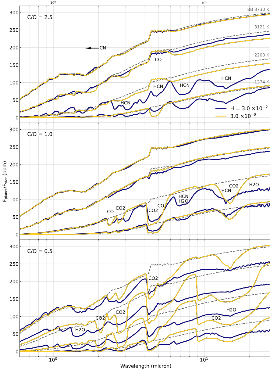
Figure 3.5: Synthetic emission spectra of a hot super-Earth with a nitrogen dominated atmosphere. The three panels represent three different C/O ratios (0.5 , 1.0 and 2.5). For each panel, 4 selected temperatures are shown, which coincide with the expected T_{\text{Peff}} of the planet ( T_{\text{Peff}} of 1274, 2200, 3121 and 3730 K). The blackbody emission for each of the temperatures is indicated with dashed grey lines. The spectra are shown with two different hydrogen mass fractions, indicated by colour.
