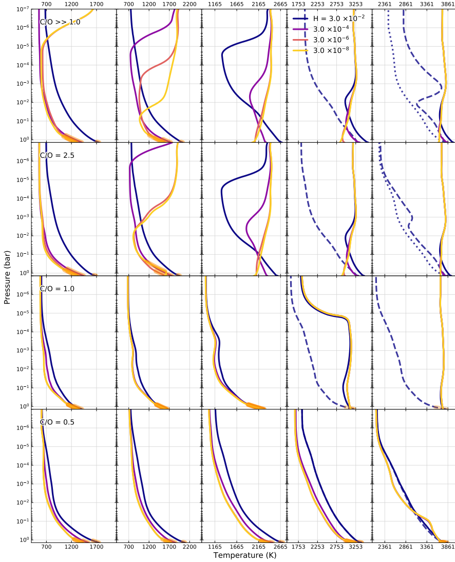
Figure 3.1: Temperature profiles in radiative-convective equilibrium computed using HELIOS for a super-Earth akin to 55 Cancri e. All cases are nitrogen-dominated and shown with varying mass fractions of hydrogen (See Table 3.1 for exact compositions). Each row represents a different C/O ratio, each column - a different orbital range (0.06, 0.04, 0.02, 0.01, 0.007 AU from left to right), hence amount of irradiation that the atmosphere experiences. For each of the cases, the profiles are shown as a function of atmospheric pressure with P_{\text{surf}} = 1.4 bar. Different colours indicate different initial abundances of hydrogen. Dashed curves show atmospheres where CN opacity was omitted. Dotted curves indicate atmospheres where CN and CH opacities were removed. Some profiles have highlighted lower regions, where convection is the dominant energy transport mechanism. The overplotted horizontal grid represents a change of one order of magnitude in pressure, vertical grid indicates intervals of 500 K in temperature. The apparent temperature inversions are caused by shortwave absorption of CN which abundance of increases with higher temperature and larger C/O ratios.
