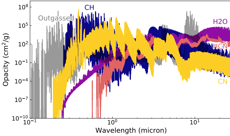
Figure 3.2: Opacity of CN in comparison with \text{H}_2\text{O} , HCN and CH for T = 2900 K and P = 1 bar. Also shown is the composite opacity of an outgassed 22 mbar magma ocean atmosphere with T = 3000 K (Zilinskas et al. in prep). For each species, the opacity is calculated assuming 100% abundance and shown at a resolution of \lambda/\Delta\lambda = 1000 .
