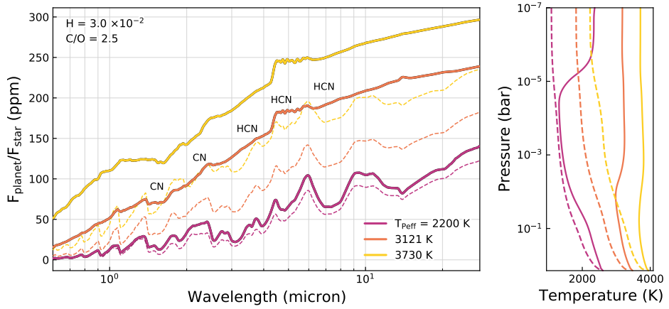
Figure 3.7: Comparison of emission spectra between atmospheres with strong shortwave absorbers (CN, CH, represented by solid curves) that cause temperature inversions and without (thin dashed lines). Shown for nitrogen dominated atmospheres with C/O = 2.5 , which is favourable for formation of CN (See Section 3.2.3). The compositions used have a hydrogen mass fraction of 3 \times 10^{-2} . Below the selected temperature range, due to inefficient CN formation, atmospheres are much less prone to temperature inversions and thus are not shown. The right panel indicates the corresponding temperature profiles.
