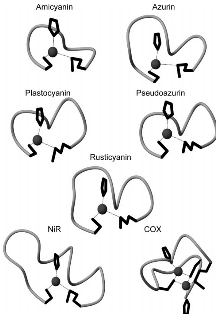
Fig. 4 Structures of the native amicyanin ligand loop and of the ligand loops 76–80 used for the loop-directed mutagenesis experiments. Although the loops of NiR 81 and COX 82 do not derive from small blue copper proteins they are included here for the sake of completeness. All loops were grafted successfully onto the \beta -sandwich structure of amicyanin to replace the native loop (shown top left).
