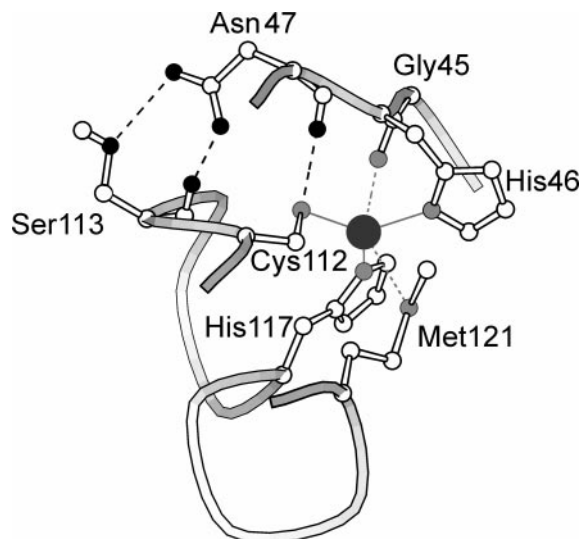
Fig. 5 Part of the structure of A. denitrificans azurin showing the participation of Asn47 in the hydrogen-bonding network connecting the two loops that contain the copper ligands. 61,79 Hydrogen bonds are indicated between Asn47 O \delta 1 and backbone proton of Ser113, Asn47 N \delta 2 and Ser 113 O \gamma 1 and between the backbone proton of Asn47 and S \delta of Cys112 (heavy dashed lines). The bonds between the copper and the equatorial ligands are indicated with the light solid lines, and the bonds between the copper and the axial ligands with light dashed lines.
