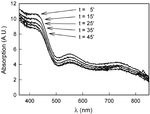
FIGURE 4: Decrease (after removal of exogenous ligands) in absorbance of oxidized NiR-H145G over time in 2 mM Mops at pH 6.5 at 15 °C. Spectra were recorded at 10 min intervals, starting 5 min after diluting a sample from a 200 mM of MOPs pH 6.5 solution one hundred times with demineralized water.
