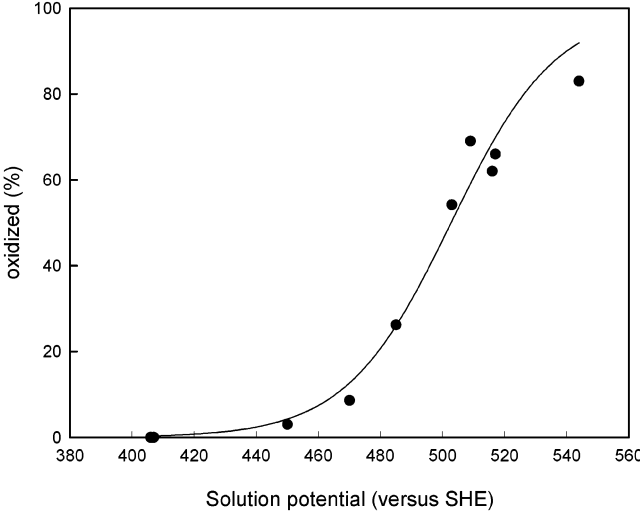
FIGURE 3: Reduction-potential of H145A-Imz. NiR H145A (10 \mu M) was incubated anaerobically overnight in a solution containing 10 mM of imidazole, 100 \mu M of \text{CuNO}_3 , and a 300 \mu M mixture of ferri/ferrocyanide. After incubation of the sample, the redox-potential of the solution was measured using a calomel electrode and the absorbance at 593 nm was determined. The percentage of oxidized protein was determined using the extinction coefficients reported in Table 3. The data were fitted to the Nernst equation to obtain a value for the redox potential.
