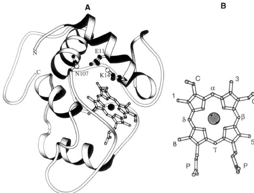
FIGURE 1: (A) Ribbon representation (Kraulis, 1991) of a model of cytc-550 based on the protein structure of P. denitrificans cytc-550 (Timkovich & Dickerson, 1976). Heme and relevant residues are in ball-and-stick representation. N and C indicate the N- and the C-terminus. (B) Heme group with the nomenclature used in this paper; \alpha , \beta , \gamma , and \delta indicate meso protons; 1, 3, 5, and 8 indicate the heme methyls (HM); P = propionate; C = position of attachment to cysteine side chain.
