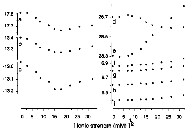
FIGURE 3: Positions (ppm) of the peaks in the 1 H-NMR spectrum ( T = 313 K) of wild-type ferricytc-550 (1.7 mM) as a function of the ionic strength ( \text{mM}^{1/2} ); a, HM5; b, HM1; c, M100 methyl; d, HM8 (open circles); e, HM3 [assignments a–e from Lommen et al. (1990)]; f–i, unassigned peaks. The ionic strength was adjusted with NaCl.
