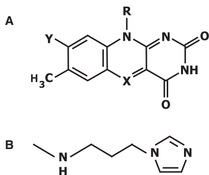
Fig. 1. (A) General structure of flavins where Y is the 8 \alpha position and R = ribityl chain. (B) In 5-deazariboflavin: X = C and Y = CH 3 . In IPAR: X = N and Y = 1-(3-aminopropyl)-imidazole.
