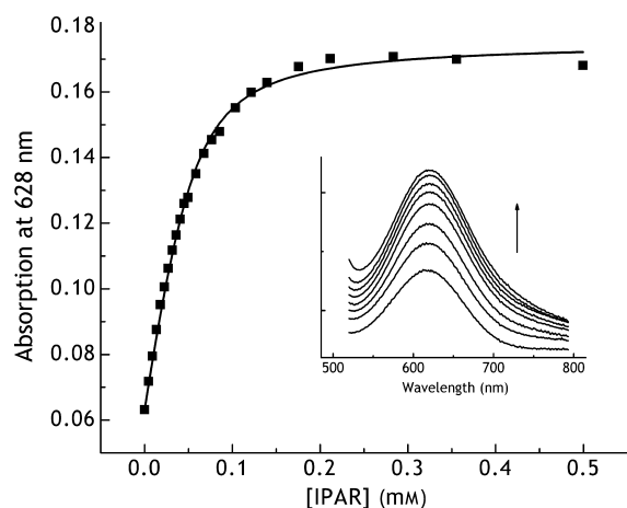
Fig. 4. The absorption at 628 nm (black squares) of a 45 \mu\text{M} aqueous solution of Cu-H117G azurin (in 20 mM Mes, pH 6.0, 25 °C) as a function of IPAR concentration, was fitted (solid line) as described previously [17], yielding a K_d^{\text{app}} of 12 \pm 1 \mu\text{M} . Inset: visible spectra of Cu-H117G azurin with increasing concentrations of IPAR (0, 18, 37, 59, 95, 124, 176 and 220 \mu\text{M} ). The arrow indicates the direction of the changes observed with increasing concentrations of IPAR.
