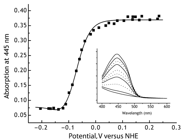
Fig. 5. Potentiometric titration of 30 \mu\text{M} of IPAR in 20 mM Mes (pH 6.0), 25 °C, fitting the absorbance changes upon oxidation and reduction at 445 nm as described in the Materials and methods. Inset: absorbance spectra showing the changes in going from the quinone to the hydroquinone and back to the quinone form of IPAR, solid lines are curves from the reductive titration, and dotted lines from the oxidative titration.
