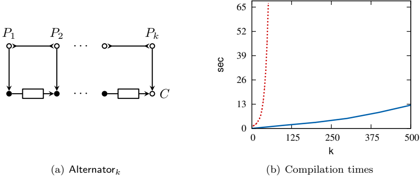
Figure 5.3: Graphical representation (a) of the \text{Alternator}_k protocol in [JKA17], for 2 \leq k \leq 500 , and its compilation time (b). The dotted red line is produced by the Jongmans' compiler (and corresponds to [JKA17, Fig 11(a)]), and the solid blue line is our compiler.
