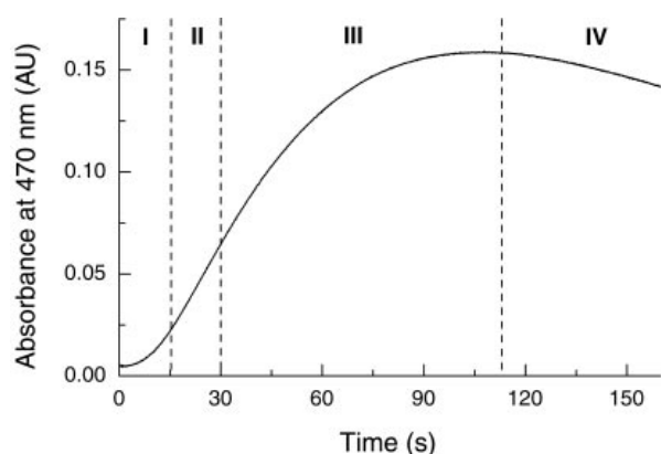
Fig. 1. A typical tetra-guaiacol formation curve. The four phases (I–IV) are described in the text. Conditions were 0.2 \mu M cytochrome c -550, 50 mM \text{H}_2\text{O}_2 and 20 mM guaiacol.
