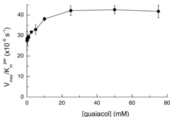
Fig. 5. Inverse slope ( V_{\text{max}}/K_{\text{m}}^{\text{per}} ) of plots of 1/\text{rate} vs. 1/[\text{H}_2\text{O}_2] as a function of [guaiacol]. [Cytochrome c -550] was 1 μM.
