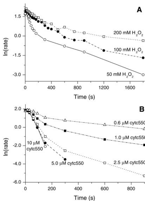
Fig. 8. Rate of the steady-state peroxidase reaction as a function of the preincubation time with H 2 O 2 . In (A), [cytochrome c -550] was 1 \mu M in the preincubation mix and [H 2 O 2 ] was varied (○, 50 mM; ●, 100 mM; □, 200 mM). In B, [H 2 O 2 ] was 50 mM in the preincubation mix and [cytochrome c -550] was varied (○, 10 \mu M; ●, 5 \mu M; □, 2.5 \mu M; ■, 1 \mu M; △, 0.6 \mu M). Activity was assayed in 10 mM guaiacol, 50 mM H 2 O 2 , and <0.5 \mu M cytochrome c -550. cytc550, cytochrome c -550.
