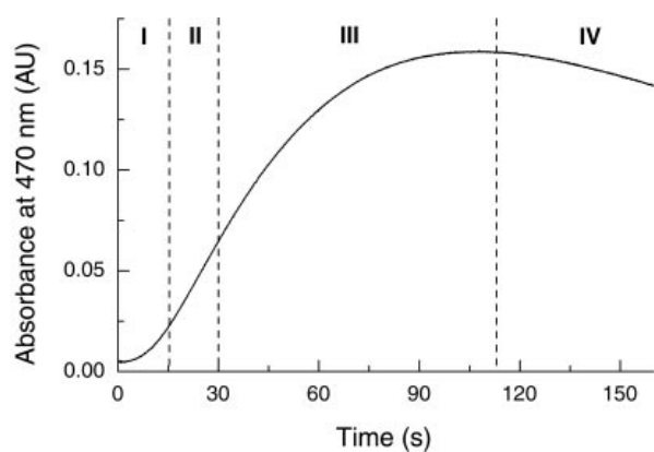
Fig. 1. A typical tetra-guaiacol formation curve. The four phases (I–IV) are described in the text. Conditions were 0.2 \mu M cytochrome c -550, 50 mM \text{H}_2\text{O}_2 and 20 mM guaiacol.
