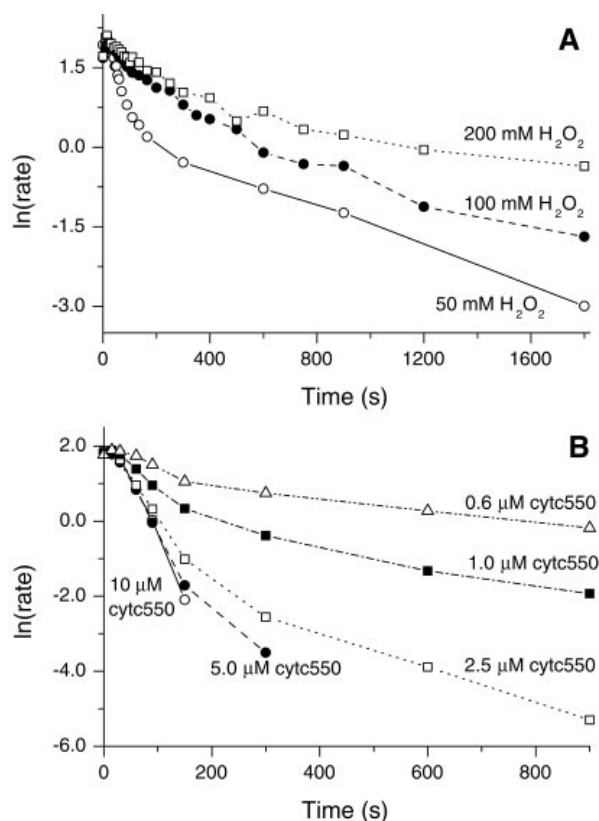
Fig. 8. Rate of the steady-state peroxidase reaction as a function of the preincubation time with \text{H}_2\text{O}_2 . In (A), [cytochrome c -550] was 1 \mu M in the preincubation mix and [\text{H}_2\text{O}_2] was varied (○, 50 mM; ●, 100 mM; □, 200 mM). In B, [\text{H}_2\text{O}_2] was 50 mM in the preincubation mix and [cytochrome c -550] was varied (○, 10 \mu M; ●, 5 \mu M; □, 2.5 \mu M; ■, 1 \mu M; △, 0.6 \mu M). Activity was assayed in 10 mM guaiacol, 50 mM \text{H}_2\text{O}_2 , and <0.5 \mu M cytochrome c -550. cyt550, cytochrome c -550.
