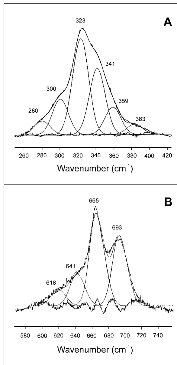
FIG. 3. Resonance Raman spectrum of H117G/N42C azurin at pH 7.5 with deconvolutions. A, low frequency range (fundamentals). B, high frequency range (combination bands). The spectrum was obtained using 413 nm excitation (25 mW), spectral resolution of 1 \text{cm}^{-1} , and 30 min of data collection. The Raman spectrum of the apo-protein was subtracted to remove the protein and glass contribution. Curves were fitted with (Gaussian) peak widths at a half-height of 21 \text{cm}^{-1} . The individual peaks and the sum of the individual peaks as well as residuals are shown.
