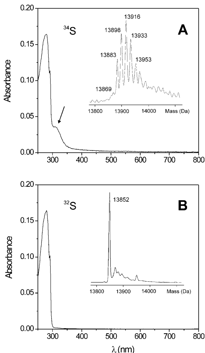
FIG. 4. UV-visible spectra and reconstituted molecular weight profile of electrospray mass spectra (insets) of H117G/N42C apoazurin. UV-visible spectra were taken in 20 mM HEPES, pH 7, at 20 °C; protein concentrations were 20 \mu M. Note the intensity of the 320 nm absorption (arrow) and the high degree of oxidation of the protein (mass spectra). A, 34 S-H117G/N42C apoazurin. B, 32 S-H117G/N42C apoazurin. The calculated masses of 34 S-H117G/N42C apoazurin and 32 S-H117G/N42C apoazurin are 13,872 and 13,852 Da, respectively.
