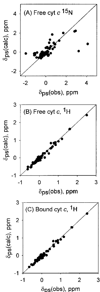
FIGURE 6: Plot of \delta_{ps}(\text{obs}) vs \delta_{ps}(\text{calc}) at 313 K for the optimized magnetic axes obtained from a five-parameter least squares search for \Gamma(\alpha, \beta, \gamma) and \Delta\chi_{\text{S}} using eq 3 for (A) ^{15}\text{N} nuclei with 77 N (set B) inputs for free cyt c , (B) ^1\text{H} nuclei with 77H N inputs (set C) for free cyt c , and (C) ^1\text{H} nuclei with 77H N inputs (set D) for bound cyt c , all fitted on 1YCC. The solid lines correspond to a perfect fit.
