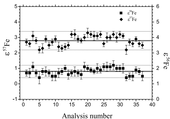
Fig. 6. Repeatability of {}^{56}\text{Fe}/{}^{54}\text{Fe} and {}^{57}\text{Fe}/{}^{54}\text{Fe} measurements. Romil Fe solution relative to IRMM-14 Fe isotope reference standard. The average Fe isotope values obtained for Romil over a period of 20 months are \epsilon^{56}\text{Fe} = 1.8 \pm 0.4 (2 S.D.) and \epsilon^{57}\text{Fe} = 2.8 \pm 0.6 (2 S.D.). This long-term repeatability is used to define an external precision of 0.4 \epsilon units for {}^{56}\text{Fe}/{}^{54}\text{Fe} and 0.6 \epsilon units for {}^{57}\text{Fe}/{}^{54}\text{Fe} measurements at 2\sigma level.
