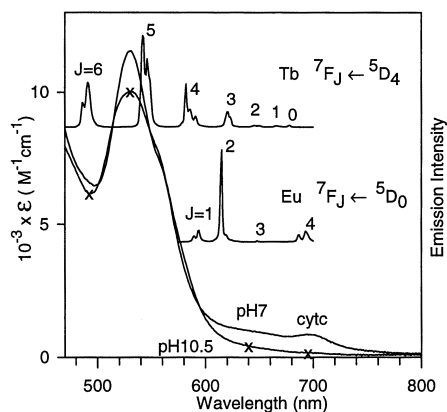
Fig. 2 Spectral overlap between the absorption spectrum of equine Fe(III) cytc at pH 7 (—) and pH 10.5 (—x—) and the emission from Tb(DPA) 3 3- and Eu(DPA) 3 3- . The assignments of the emission bands are also given
