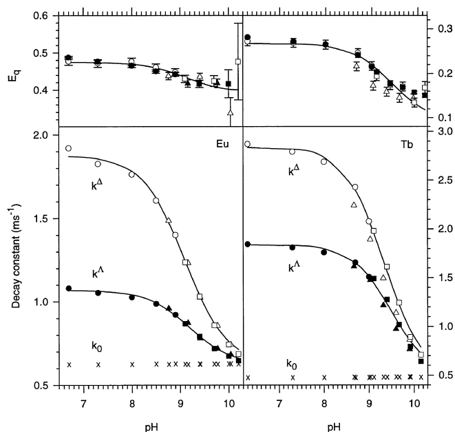
Fig. 1 pH dependence of the decay constants of \text{Ln}(\text{DPA})_3^{3-} luminescence in the absence ( k_0 ) and in the presence ( k^\Delta , k^\Lambda ) of ferricyte (lower part), and values of E_q (upper part). The shape of the symbols for the data points relates to the buffer (10 mM) used: Tris ( \circ ), ethanolamine ( \Delta ), Ches ( \square ). In the bottom plots, fits of Eq. 7 to the experimental data are shown as solid lines; fit parameters can be found in Table 1. The symbols used to represent E_q data have the following meaning: open symbols pertain to values from decay measurements; solid symbols to values from g_{\text{lum}}^{\text{cw}} measurements (see text). The error bars show the standard error of E_q . The solid line is not a fit to the E_q data points but is obtained by calculation of E_q from the fits to k^\Delta and k^\Lambda shown in the lower part of the graph. Sample conditions: [\text{Ln}] = 1 \text{ mM} , [ferricyte] = 11 \mu\text{M} , ionic strength I = 22 \text{ mM} (kept constant by addition of NaCl)
