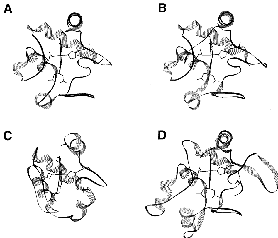
FIGURE 1: Schematic representation of the crystal structures of the c-type cytochromes used in this study. Panels A–D respectively depict horse heart cytc (54), yeast iso-1-cytc C102T (55), Ps. aeruginosa cytc-551 (56), and P. denitrificans cytc-550 (57). Although no structure has yet been solved for P. versutus cytc-550, it is thought to be very similar to the highly homologous cytc-550 from P. denitrificans (58).
