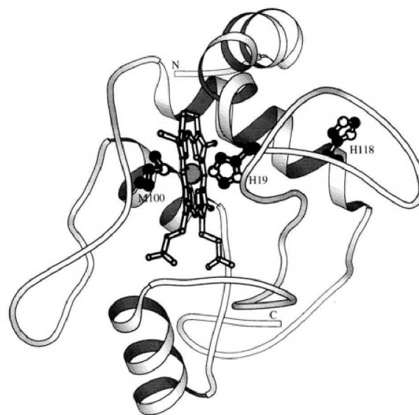
FIGURE 1: Ribbon representation (Kraulis, 1991) of a model of cytc-550 based on the protein structure of P. denitrificans cytc-550 (Timkovich & Dickerson, 1976). Heme and relevant residues are in ball-and-stick representation. N, and C indicate N- and C-terminus.
