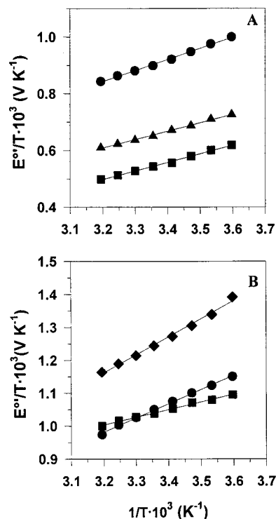
FIGURE 2: E^\circ/T vs 1/T plots for wild-type and mutated azurins at pH 7. The slope of the plots yields the -\Delta H_{\text{rc}}^{\circ} values. (A) A. denitrificans azurin: wild type (●), M121Q (■), and M121H (▲). (B) P. aeruginosa azurin: wild type (●), H35L (■), and M44K (◆). Conditions: protein concentration, 0.1 mM; base electrolyte, 0.1 M phosphate, pH 7. Solid lines are least-squares fits to the data points. Error bars have the same dimensions of the symbols.
