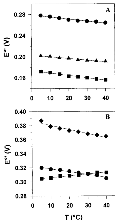
FIGURE 1: E^\circ vs T plots for wild-type and mutated azurins at pH 7. The slope of the plots yields the \Delta S_{\text{rc}}^{\circ} values. (A) A. denitrificans azurin: wild type (●), M121Q (■), and M121H (▲). (B) P. aeruginosa azurin: wild type (●), H35L (■), and M44K (◆). Conditions: protein concentration, 0.1 mM; base electrolyte, 0.1 M phosphate, pH 7. Solid lines are least-squares fits to the data points. Error bars have the same dimensions of the symbols.
