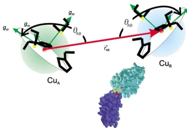
Figure 1. Structure of az-1 dimer. Schematic representation: Relative orientation of the two copper sites \text{Cu}_A and \text{Cu}_B in the dimer as well as the principal axes of the g tensor with respect to the ligands. \vec{r}_{AB} : vector between \text{Cu}_A and \text{Cu}_B ; \theta_{AB} : dipolar angle for B_0 in the g_{xx} – g_{yy} plane. Insert: space-filling model of the dimer structure from X-ray crystallography. [4]
