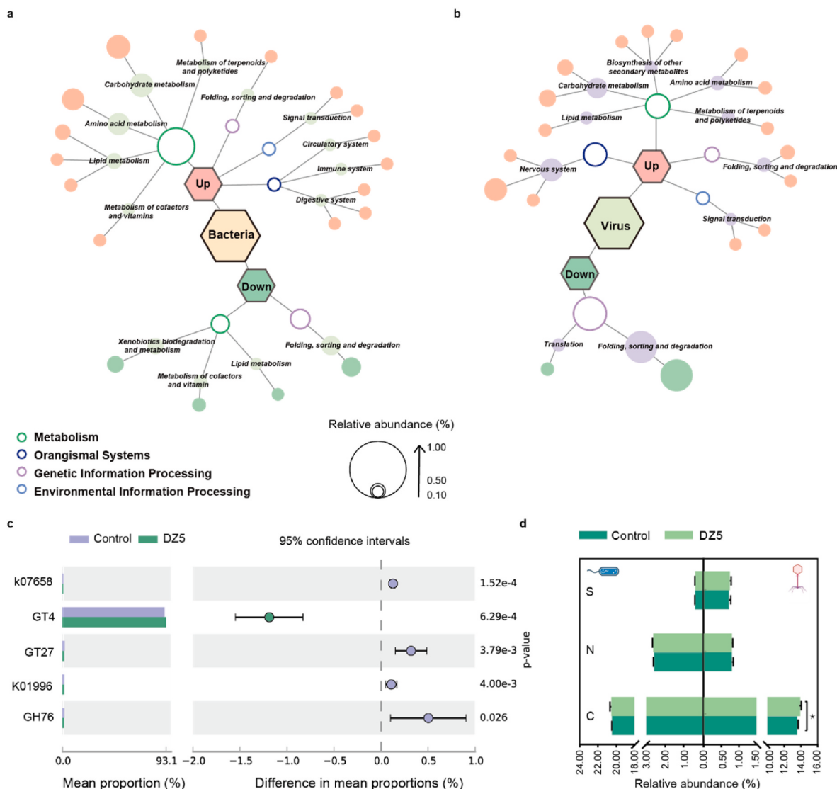
Fig. 5. Soil metagenomes revealed effects of difenoconazole exposure on soil function. Based on level 3 in the KEGG database enrichment of significantly altered soil bacterial community and viral community functional potential in DZ5-treated group compared with control, the size of the bubble is controlled as a reference (a, b). Differential abundance analysis of microbiome functional genes in the DZ5-treated group compared with control (c). The enrichment of bacterial and viral genes encoding CNS metabolic functions (d).
