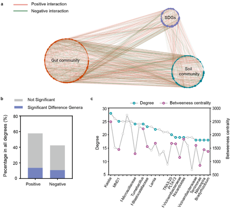
Fig. 3. Co-occurrence network analysis revealing the correlation between significantly different genera and soil-gut bacterial communities, the size of the node was determined according to the degree of each genus, SDGs: significantly different genera (a). The proportion of significantly different genera with positive and negative correlations in the whole community (b). According to soil-soil fauna gut network analysis to investigate the degree and betweenness centrality of significantly different genera (c).
