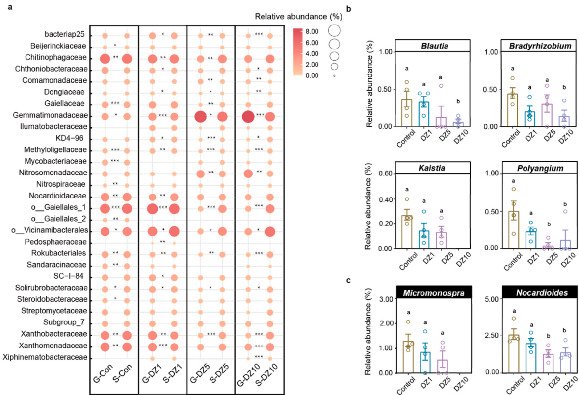
Fig. 2. Shared bacterial families (the relative abundance >1%) between E. crypticus gut and soil groups, G:gut; S:soil. (a). Decreased relative abundance of beneficial bacteria in gut (white background) and soil (black background) after exposure, respectively (b, c). * P < 0.05 , ** P < 0.01 , and *** P < 0.001 , represents the significant difference between gut and soil treatments (two-tailed Welch's t -test, P < 0.05 ). The letters represent differences between various treatment groups by one-way ANOVA with Tukey's post-hoc test, P < 0.05 .
