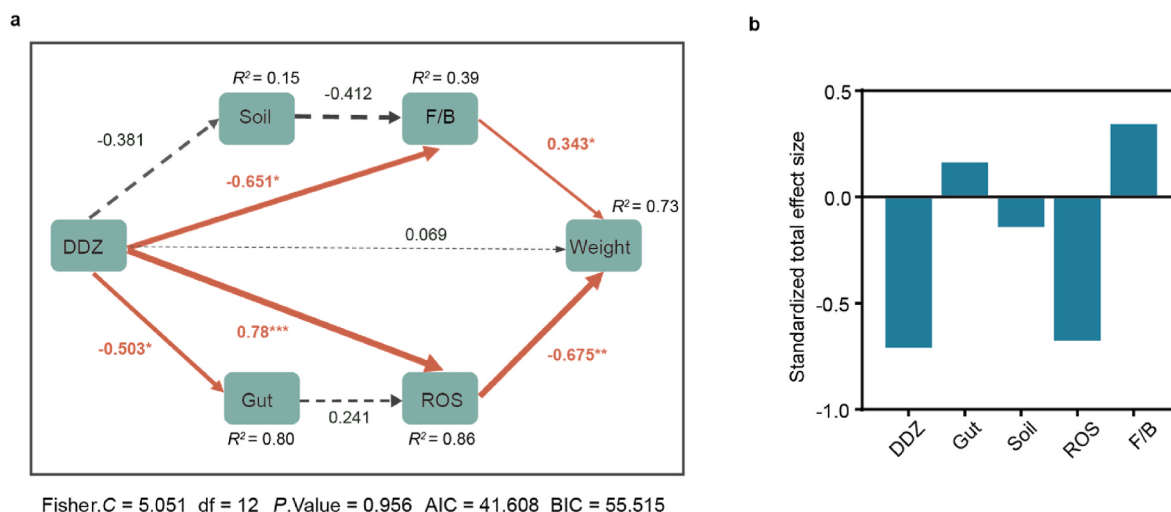
Fig. 4. SEM was applied to evaluate the relationship between difenoconazole exposure dose, soil bacteria (PCoA1 of Bray-Curtis distance), gut bacteria (PCoA1 of Bray-Curtis distance), ROS, F/B (the ratio about the relative abundances of Firmicutes and Bacteroidetes in gut bacteria) and weight of E. crypticus . The number on the line represents the path coefficient, which is proportional to the width of the arrow, the R^2 represents the proportion of variance explained. Solid and dashed lines reflect significant and insignificant correlations, respectively (a). Plot showing the total normalized effect of the above indicators on body weight (b).
