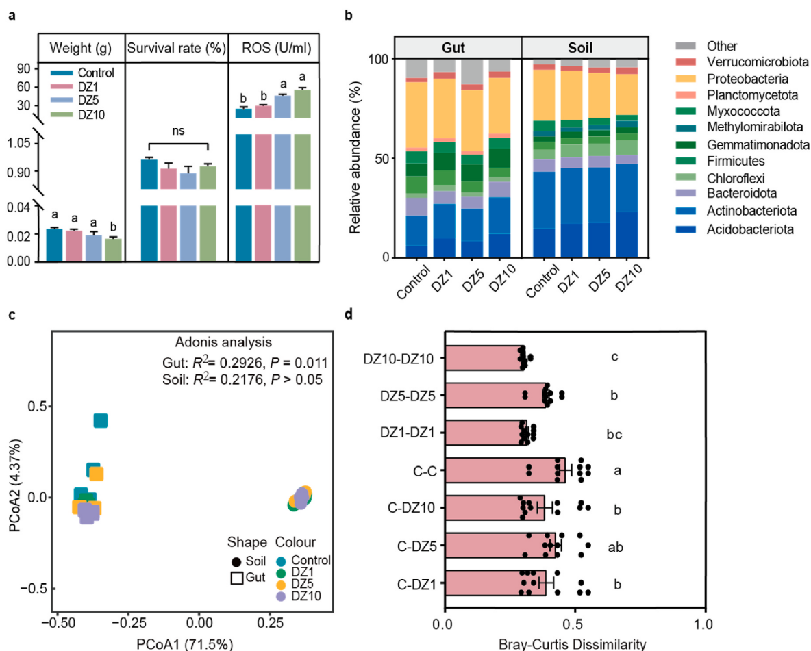
Fig. 1. Effects of difenoconazole exposure on body weight, survival rate, and reactive oxygen species (ROS) concentrations of E. crypticus in treated groups (a). Relative abundance of phylum (top 10) in gut and soil bacterial communities (b). PCoA based on genus level revealed significant separation of soil and gut bacterial communities (c). Intragroup and intergroup differences of gut bacterial communities based on Bray-Curtis dissimilarity (d). The letters represent differences between various treatment groups by one-way ANOVA with Tukey's post-hoc test, P < 0.05 .
