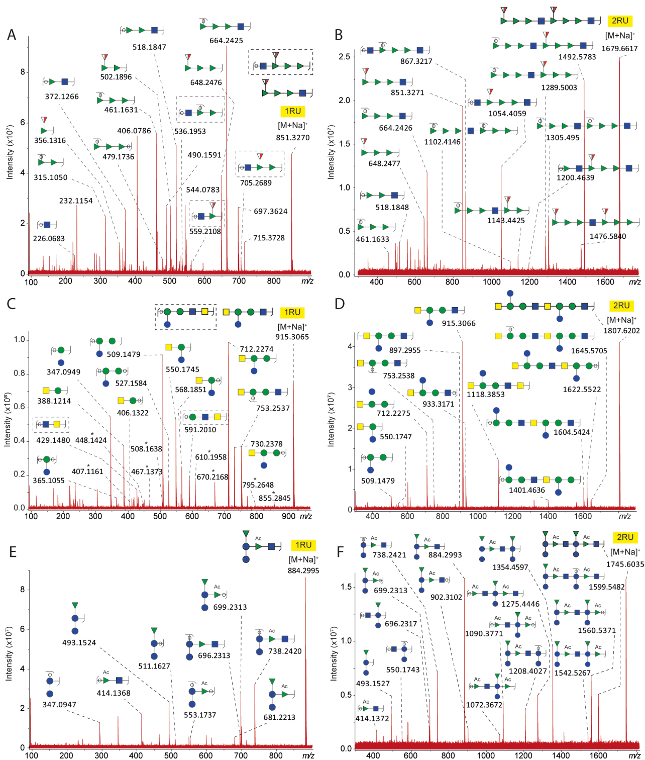
Figure 5. MALDI-MS/MS CID FT-ICR tandem mass spectra of the sodiated B fragment ion corresponding to 1RU and 2RU of the glycoconjugates EcoO2 (A and B), EcoO6A (C and D), and EcoO25B (E and F). For many species, several isomeric structures are possible of which only a single one is displayed. *Cross-ring fragment ions.
