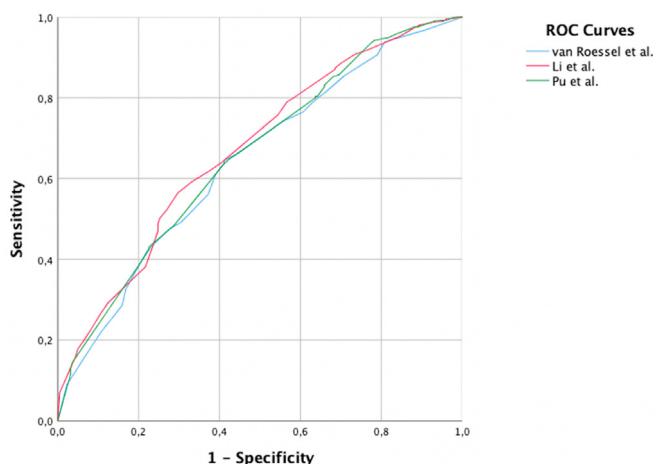
Fig. 3. ROC curves for 3-year OS for the 3 nomograms (areas under curve: 0.644 for the nomogram by van Roessel et al., 0.655 for the nomogram by Pu et al., and 0.665 for the nomogram by Li et al.).
