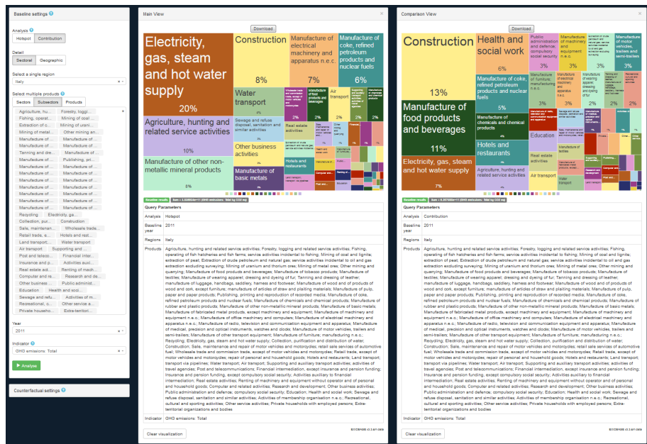
Figure 3: Sectoral hotspot (on the left) and contribution (on the right) analysis of GHG emissions in Italy
