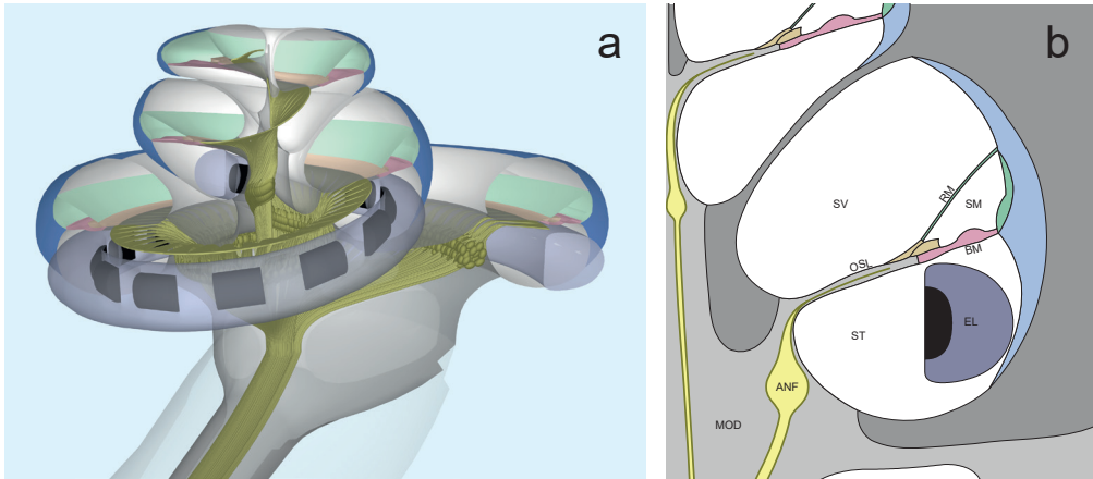
Figure 1.2. Schematic overview of select structures inside the (human) cochlea. Panel a shows a partial cross-section of a cochlea from the computational model central to this thesis. Panel b shows a line drawing of the cross-section at the beginning of the second turn of the cochlea. The main compartments denoted are the scala vestibuli (SV), scala media (SM) and scala tympani (ST), the latter of which contains the electrode array (EL). These compartments are separated by the osseous spiral lamina (OSL), basilar membrane (BM) and Reissner's membrane (RM). Also depicted are the auditory nerve fibres (ANF), which run through the osseous spiral lamina and the cochlear modiolus (MOD).
