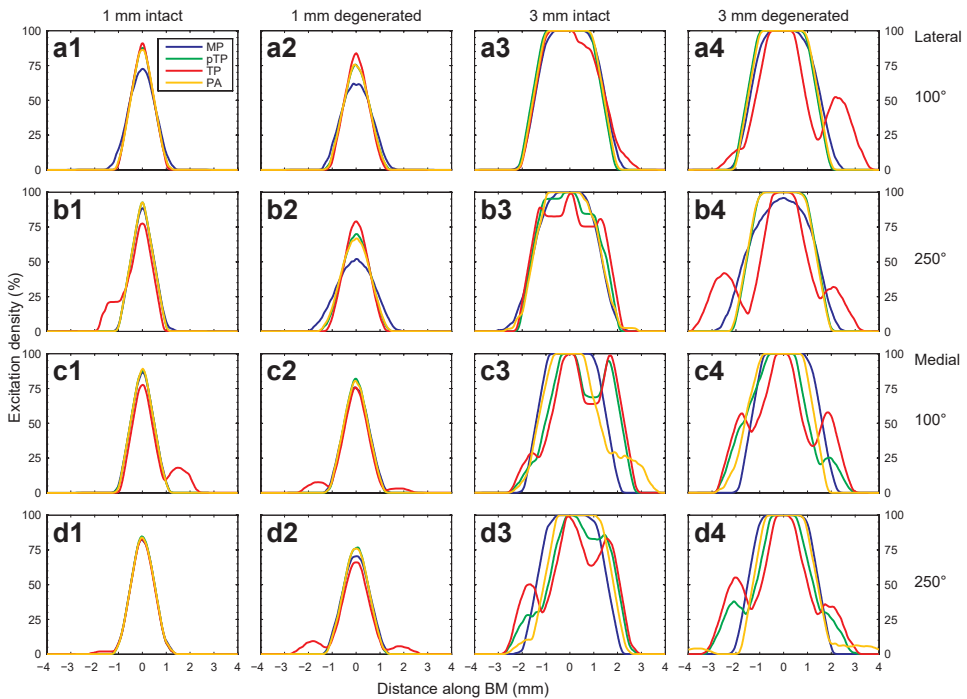
Figure 6.5. ED plots of the XPs in figure 6.4. The abscissa represents position along the BM, centred on the peak of the ED curves, the ordinate represents the percentage of excited neurons in a 1 mm segment at a given position of the BM. Rows a and b correspond to lateral contacts at 100° and 250° insertion depth respectively, rows c and d correspond to medial contacts at the same angles.; column 1 consists of ED curves at 1 mm excitation width from simulations with intact neurons, column 2 is the same but from simulations with neurons that had degenerated peripheral processes. Columns 3 and 4 consist of ED plots at 3 mm excitation width, with intact and degenerated neurons respectively. Blue curves represent MP stimulation, green represents pTP, red TP and orange corresponds to PA stimulation.
