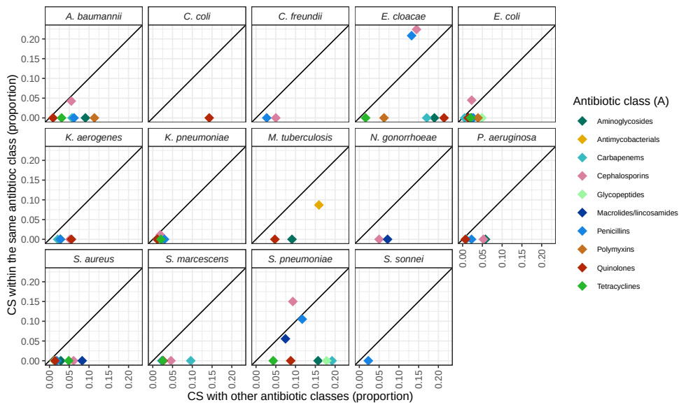
Figure S6.2: Collateral sensitivity (CS) between antibiotic classes. The proportion of CS effects detected within and between antibiotic classes for each species ( C. jejuni was excluded, because there were no collateral effects estimated within the antibiotic class). On the x-axis the proportion of detected CS effects with other antibiotic classes. On the y-axis the proportion of detected CS effects within the same antibiotic class. The line denotes no difference between CS detected within and between antibiotic classes. All antibiotic classes in the lower right triangle more often show CS with other classes than within their own antibiotic class.
