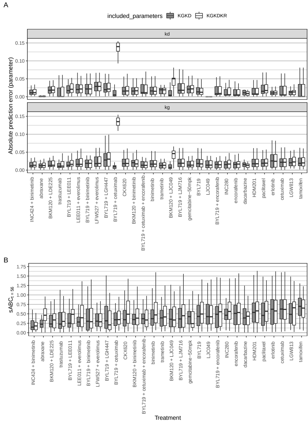
Figure S3.3: The prediction errors for the two models with (white) and without (grey) inclusion of k_r in the multivariate lasso for all treatments where the k_r was estimated non-zero in the non-linear mixed effect estimation. A) the absolute prediction error of the parameter values. B) the sABC for the same treatments. Both the prediction errors and the sABC are generally higher for the lasso without inclusion of k_r .
