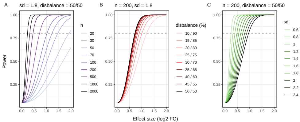
Figure 5.5: Properties of the collateral effects detection. Power analysis for t-test of collateral effects against the mean \log_2 FC. The power against effect size. A) Power for different sample sizes ( n ), lighter colors show lower n . Power increases greatly with n . B) Power for different disbalances in the group sample sizes. The most equal groups are divided 50/50, while 10/90 shows a large disbalance in sample sizes, which shows decreased power. C) The power for different standard deviations of the MIC distributions.
