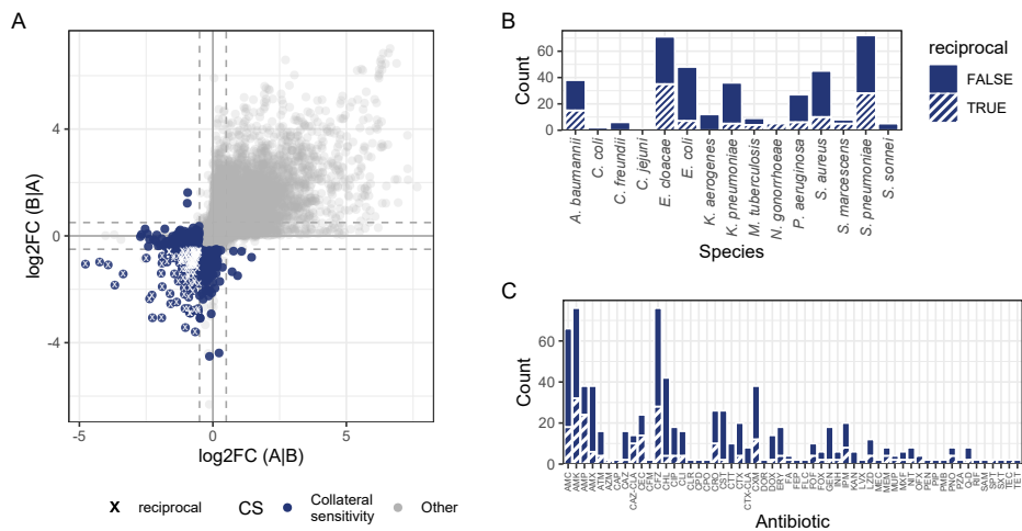
Figure 6.3: Overview of estimated collateral effects and reciprocity across species. A) Estimated effect sizes (log 2 fold change (FC)) of the MIC of reciprocal and non-reciprocal collateral sensitivity responses and other responses, no collateral effect and collateral resistance. Antibiotic A and B represent an antibiotic pair, for which the effect size in both directions is estimated, A given dichotomization on B ( A | B ) and, B given dichotomization on A ( B | A ). Dashed lines denote the threshold of relevant effect sizes (abs(log 2 FC = 0.5). B) Number of collateral sensitivity effects for each species and whether they are reciprocal (striped) or not (blue). C) Number of collateral sensitivity effects for each antibiotic. Note that every collateral sensitivity effect contributes to two antibiotics.
